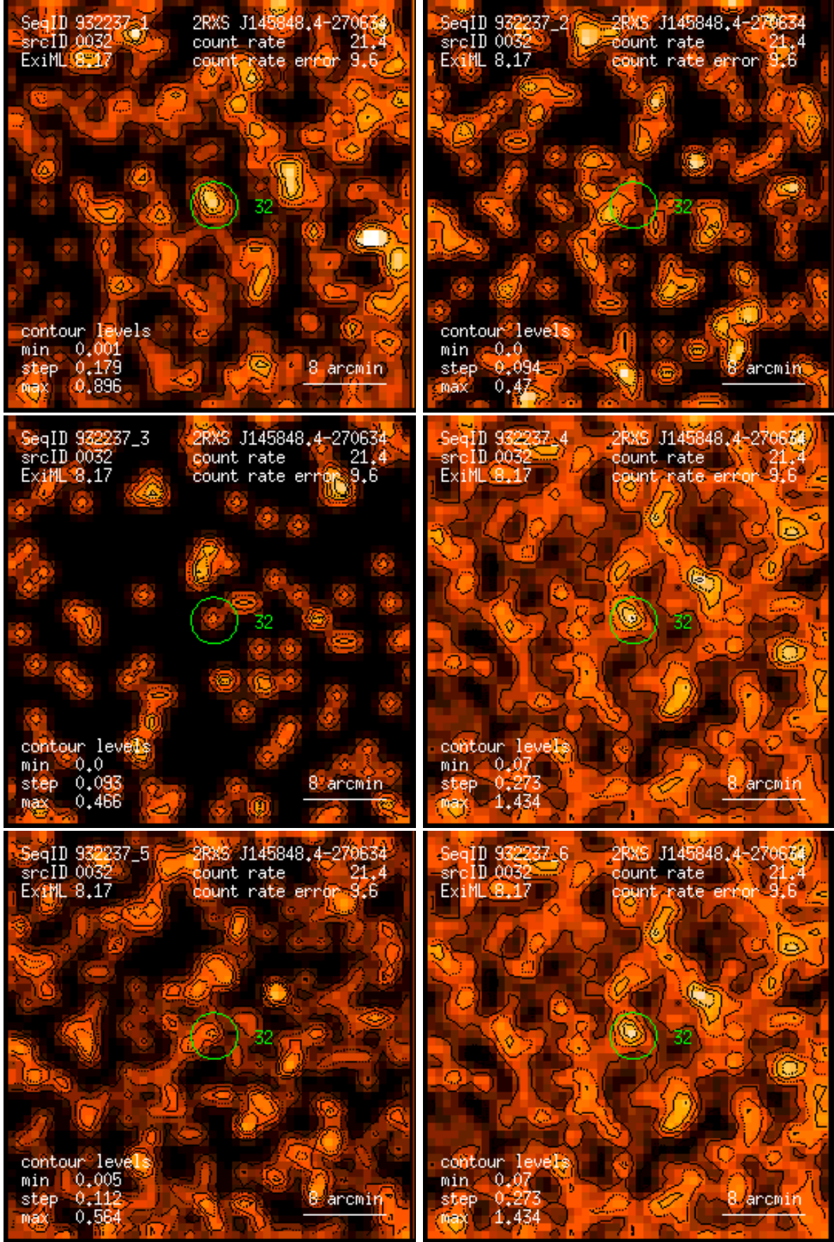
Figure 32: RASS 932237: detection 0032: band rate images, Gaussian filter: (1) PSPC channels 11 – 41, (2) 52 – 90, (3) 91 – 201, (4) 11 – 235, (5) 52 – 201, (6) 11 – 201. Broad band rates in counts/ks. Band rate contour levels in counts/ks/arcmin 2 .
