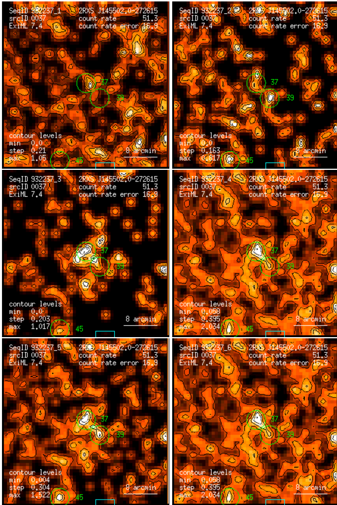
Figure 37: RASS 932237: detection 0037: band rate images, Gaussian filter: (1) PSPC channels 11 – 41, (2) 52 – 90, (3) 91 – 201, (4) 11 – 235, (5) 52 – 201, (6) 11 – 201. Broad band rates in counts/ks. Band rate contour levels in counts/ks/arcmin 2 .
