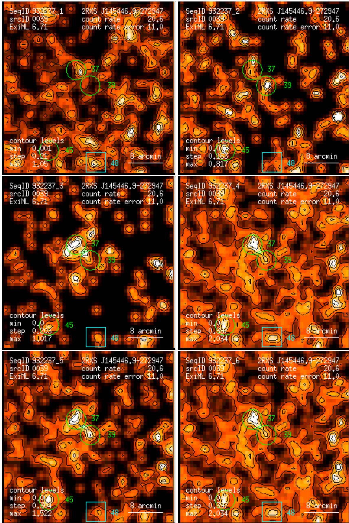
Figure 39: RASS 932237: detection 0039: band rate images, Gaussian filter: (1) PSPC channels 11 – 41, (2) 52 – 90, (3) 91 – 201, (4) 11 – 235, (5) 52 – 201, (6) 11 – 201. Broad band rates in counts/ks. Band rate contour levels in counts/ks/arcmin 2 .
