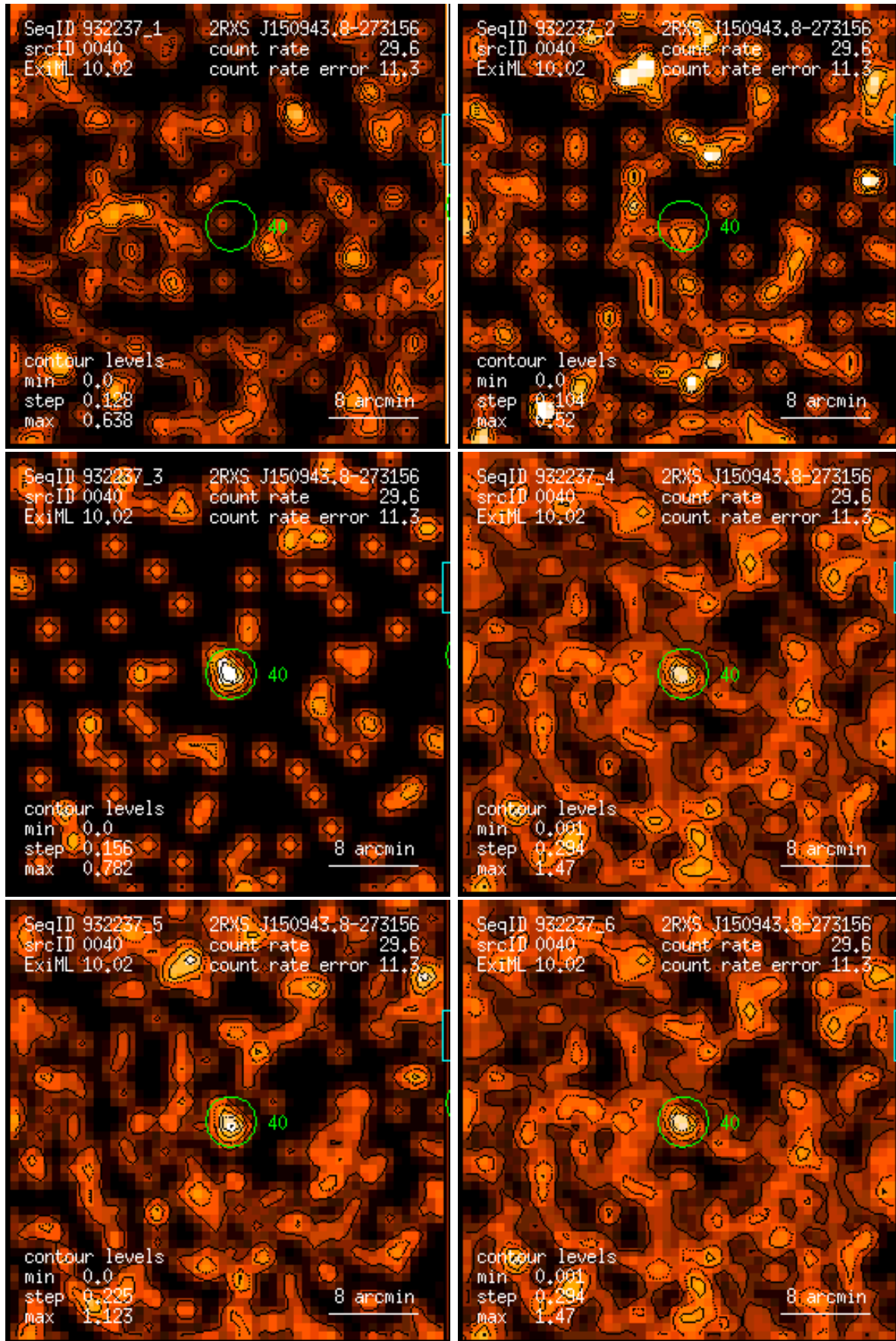
Figure 40: RASS 932237: detection 0040: band rate images, Gaussian filter: (1) PSPC channels 11 – 41, (2) 52 – 90, (3) 91 – 201, (4) 11 – 235, (5) 52 – 201, (6) 11 – 201. Broad band rates in counts/ks. Band rate contour levels in counts/ks/arcmin 2 .
