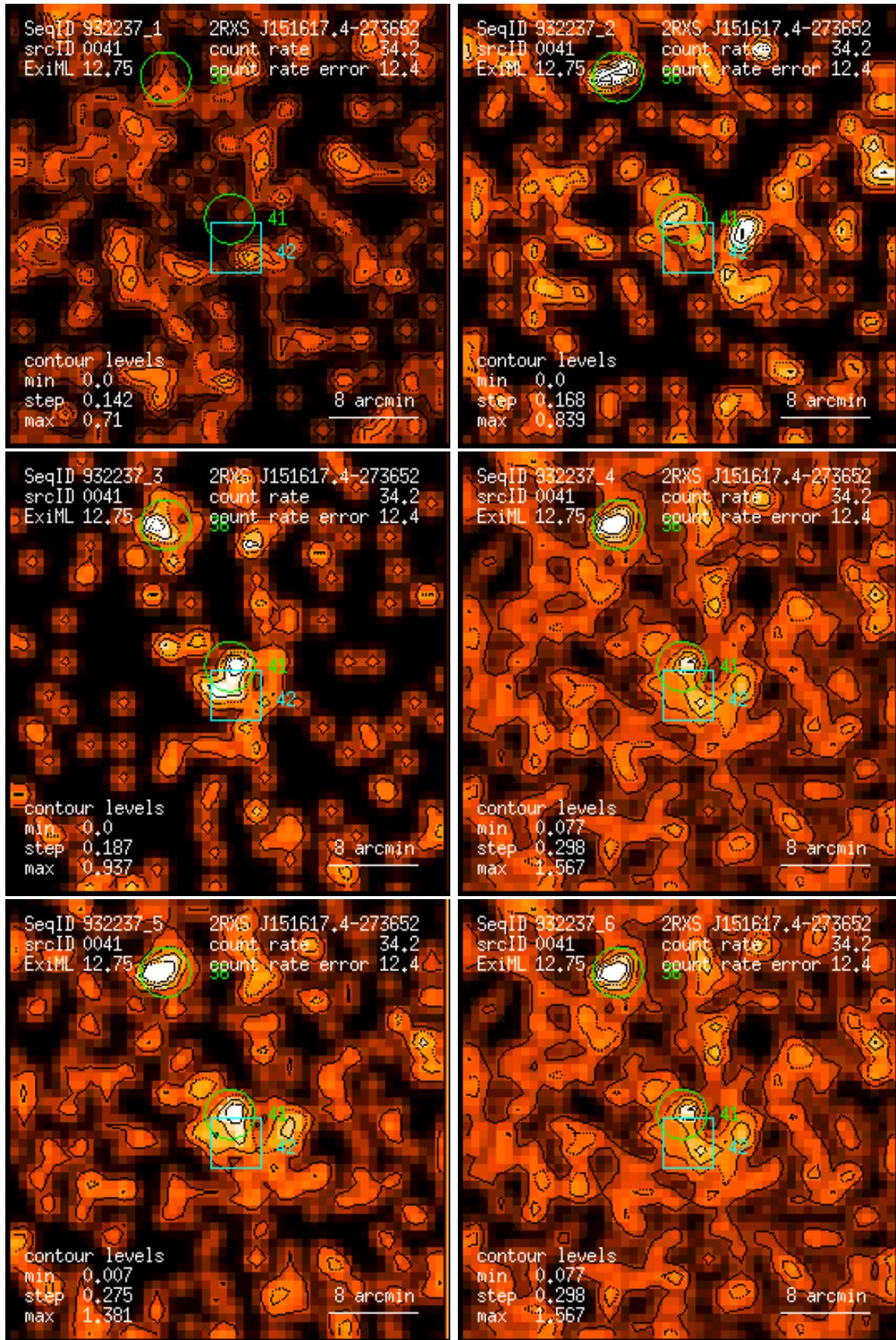
Figure 41: RASS 932237: detection 0041: band rate images, Gaussian filter: (1) PSPC channels 11 – 41, (2) 52 – 90, (3) 91 – 201, (4) 11 – 235, (5) 52 – 201, (6) 11 – 201. Broad band rates in counts/ks. Band rate contour levels in counts/ks/arcmin 2 .
