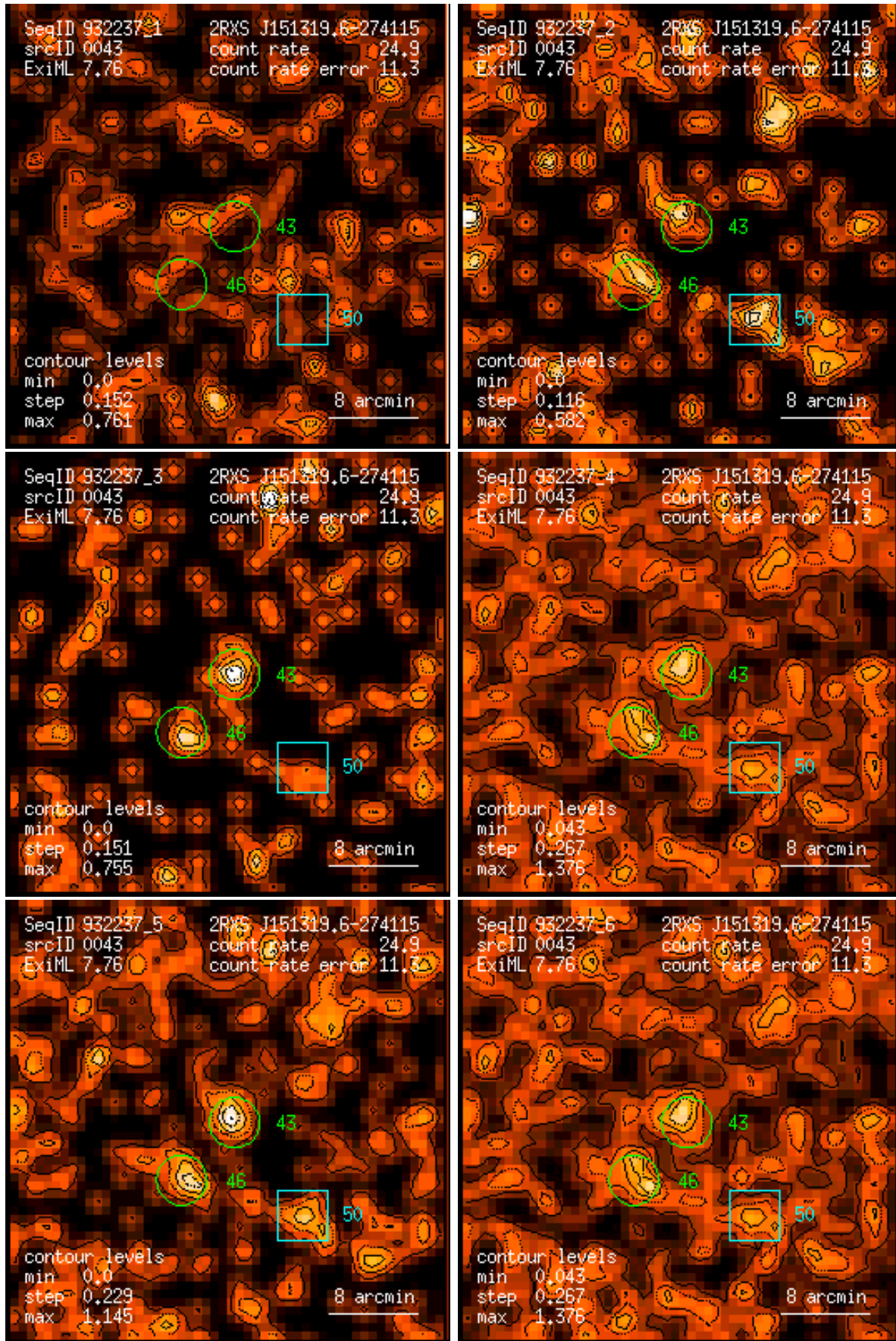
Figure 43: RASS 932237: detection 0043: band rate images, Gaussian filter: (1) PSPC channels 11 – 41, (2) 52 – 90, (3) 91 – 201, (4) 11 – 235, (5) 52 – 201, (6) 11 – 201. Broad band rates in counts/ks. Band rate contour levels in counts/ks/arcmin 2 .
