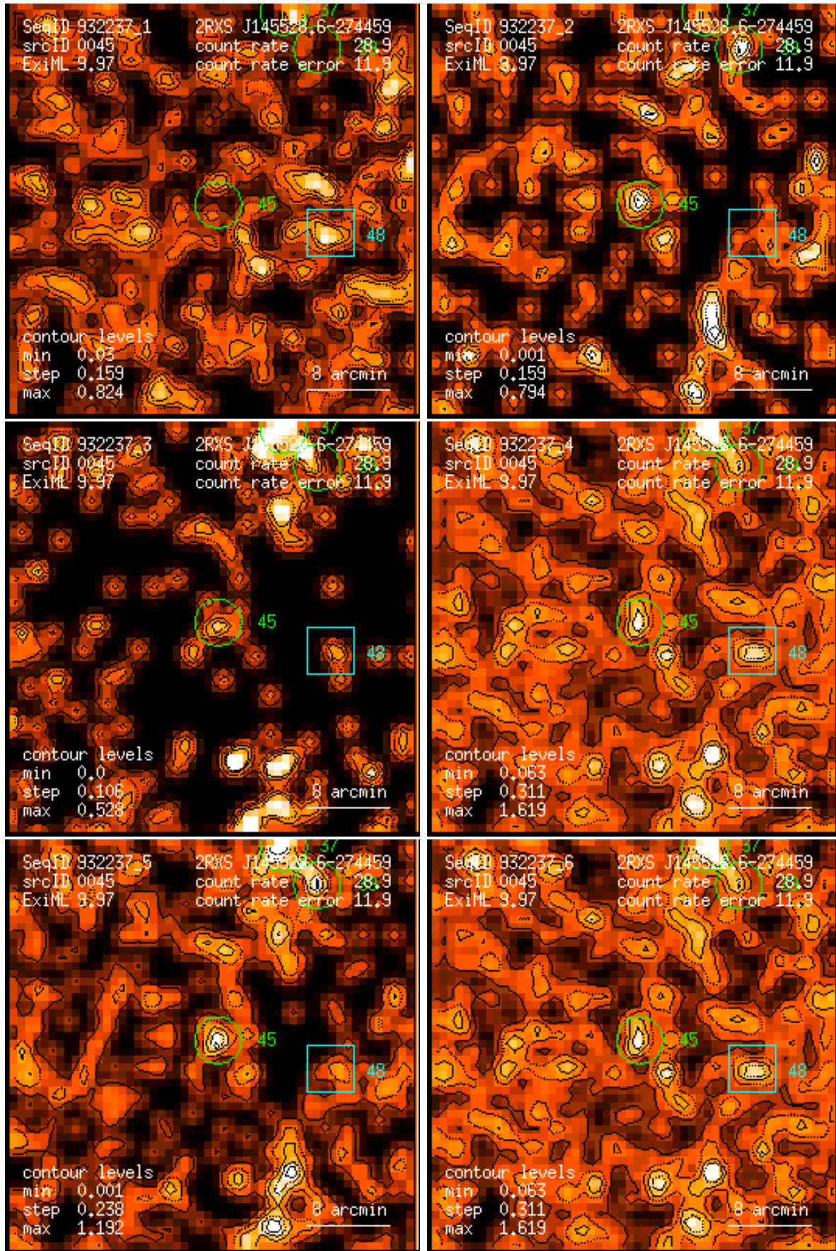
Figure 45: RASS 932237: detection 0045: band rate images, Gaussian filter: (1) PSPC channels 11 – 41, (2) 52 – 90, (3) 91 – 201, (4) 11 – 235, (5) 52 – 201, (6) 11 – 201. Broad band rates in counts/ks. Band rate contour levels in counts/ks/arcmin 2 .
