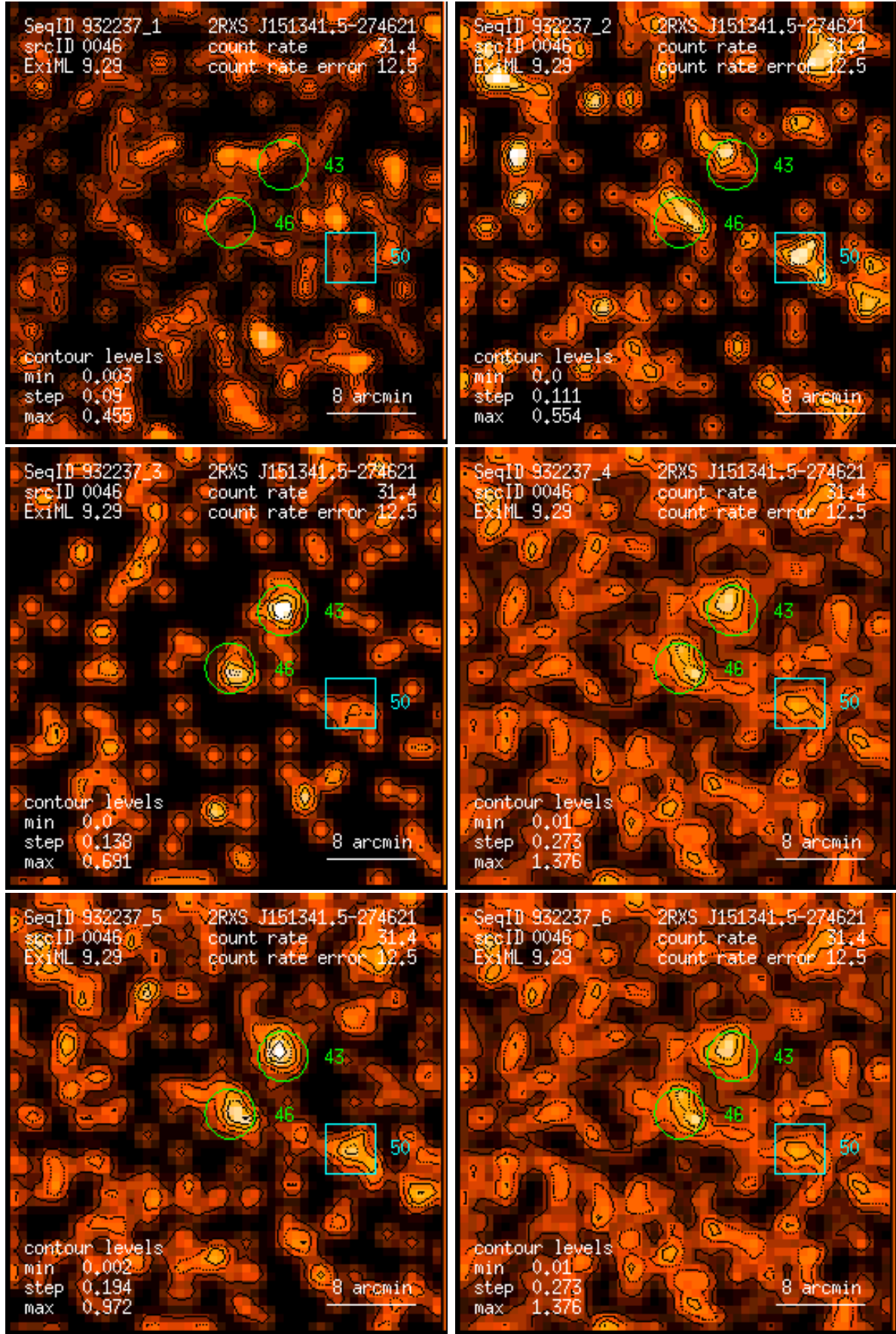
Figure 46: RASS 932237: detection 0046: band rate images, Gaussian filter: (1) PSPC channels 11 – 41, (2) 52 – 90, (3) 91 – 201, (4) 11 – 235, (5) 52 – 201, (6) 11 – 201. Broad band rates in counts/ks. Band rate contour levels in counts/ks/arcmin 2 .
