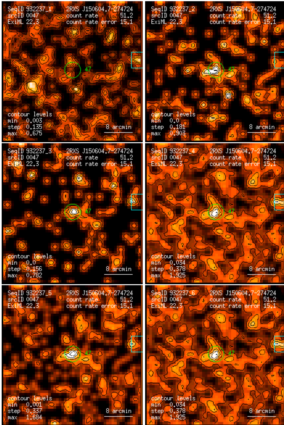
Figure 47: RASS 932237: detection 0047: band rate images, Gaussian filter: (1) PSPC channels 11 – 41, (2) 52 – 90, (3) 91 – 201, (4) 11 – 235, (5) 52 – 201, (6) 11 – 201. Broad band rates in counts/ks. Band rate contour levels in counts/ks/arcmin 2 .
