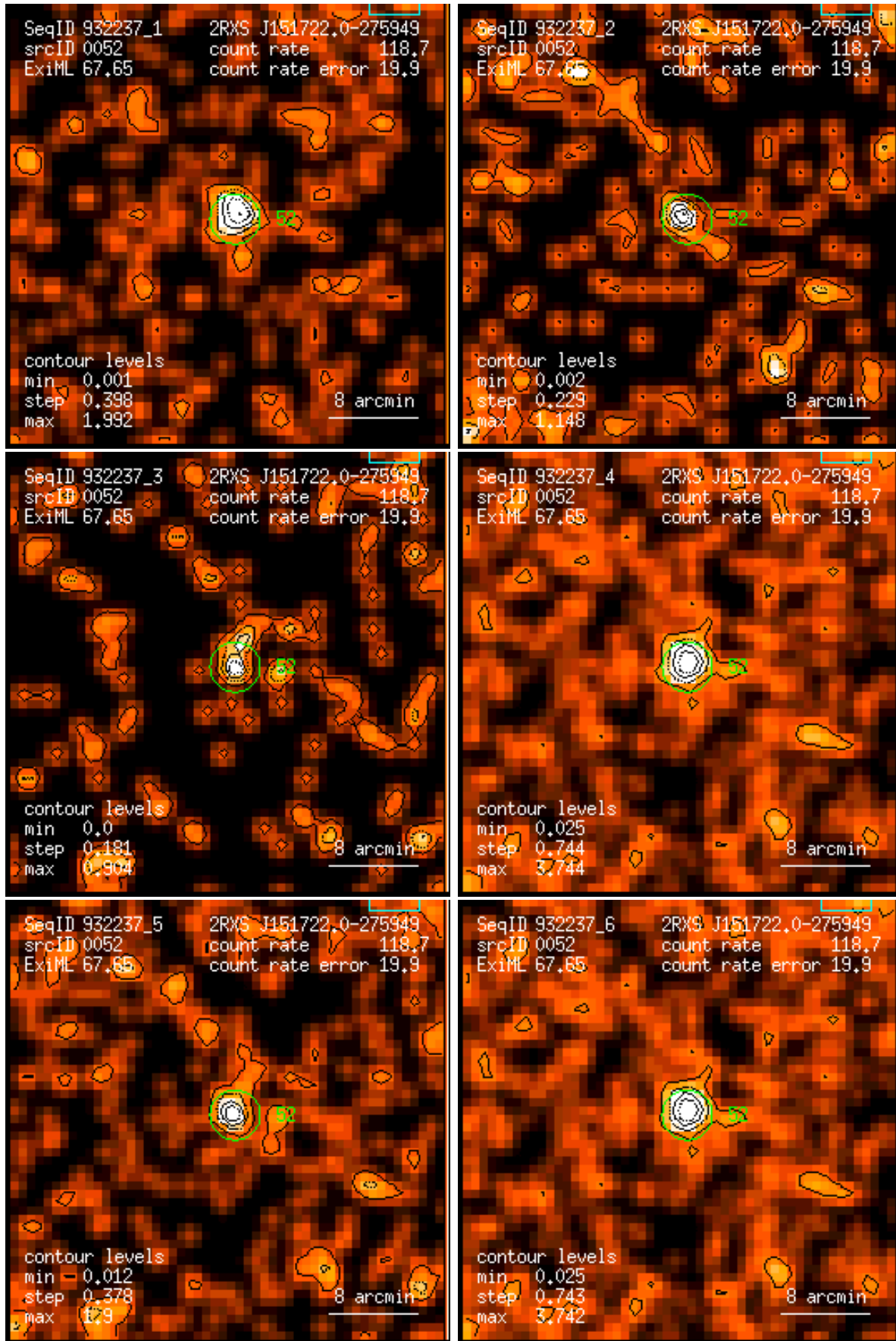
Figure 52: RASS 932237: detection 0052: band rate images, Gaussian filter: (1) PSPC channels 11 – 41, (2) 52 – 90, (3) 91 – 201, (4) 11 – 235, (5) 52 – 201, (6) 11 – 201. Broad band rates in counts/ks. Band rate contour levels in counts/ks/arcmin 2 .
