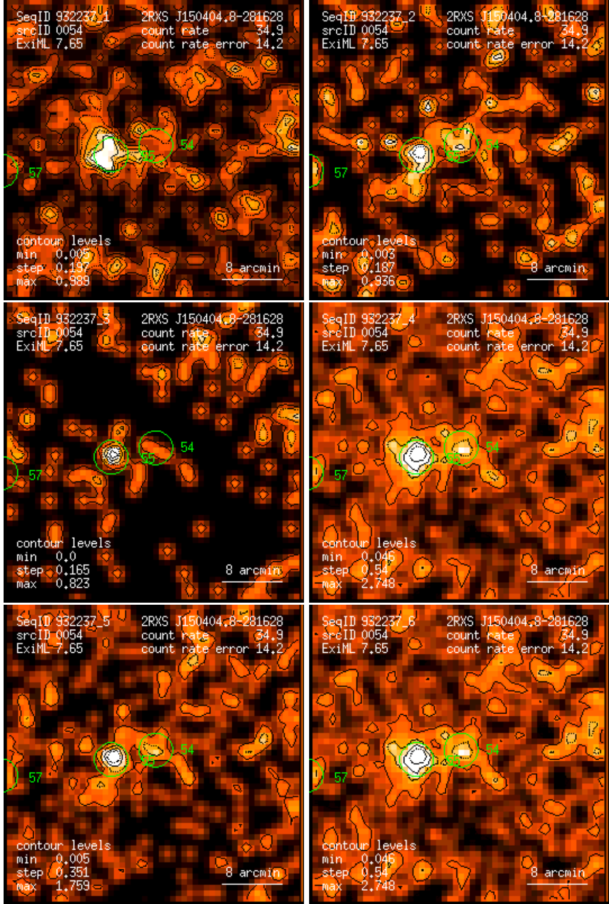
Figure 54: RASS 932237: detection 0054: band rate images, Gaussian filter: (1) PSPC channels 11 – 41, (2) 52 – 90, (3) 91 – 201, (4) 11 – 235, (5) 52 – 201, (6) 11 – 201. Broad band rates in counts/ks. Band rate contour levels in counts/ks/arcmin 2 .
