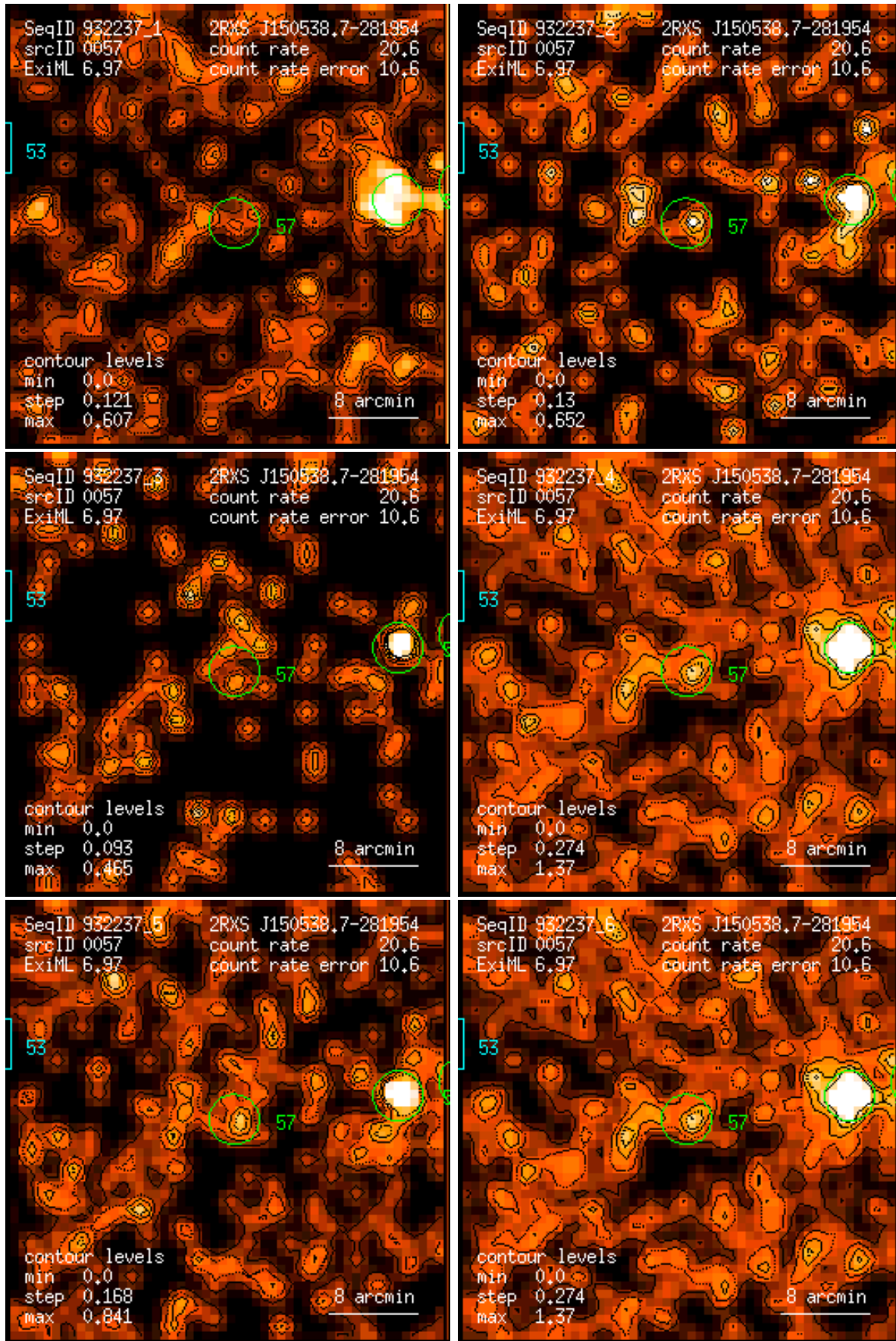
Figure 57: RASS 932237: detection 0057: band rate images, Gaussian filter: (1) PSPC channels 11 – 41, (2) 52 – 90, (3) 91 – 201, (4) 11 – 235, (5) 52 – 201, (6) 11 – 201. Broad band rates in counts/ks. Band rate contour levels in counts/ks/arcmin 2 .
