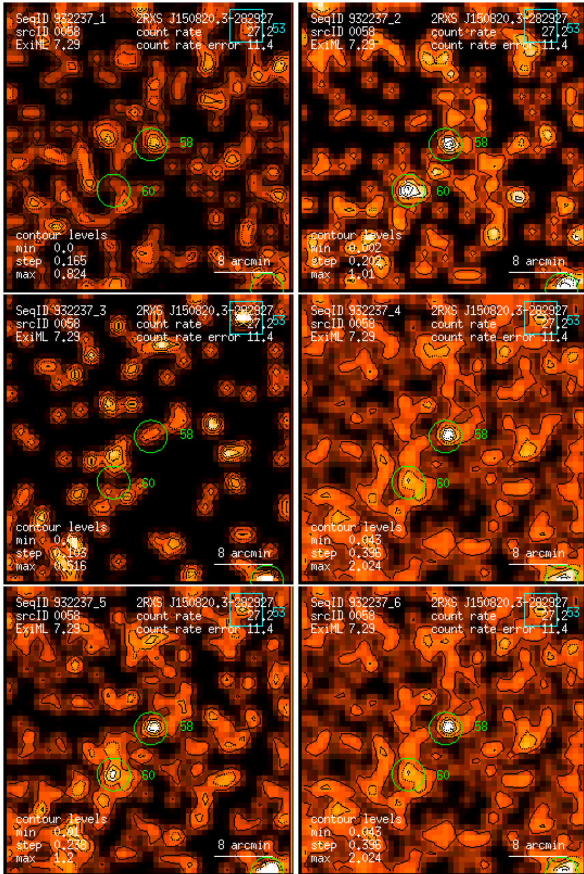
Figure 58: RASS 932237: detection 0058: band rate images, Gaussian filter: (1) PSPC channels 11 – 41, (2) 52 – 90, (3) 91 – 201, (4) 11 – 235, (5) 52 – 201, (6) 11 – 201. Broad band rates in counts/ks. Band rate contour levels in counts/ks/arcmin 2 .
