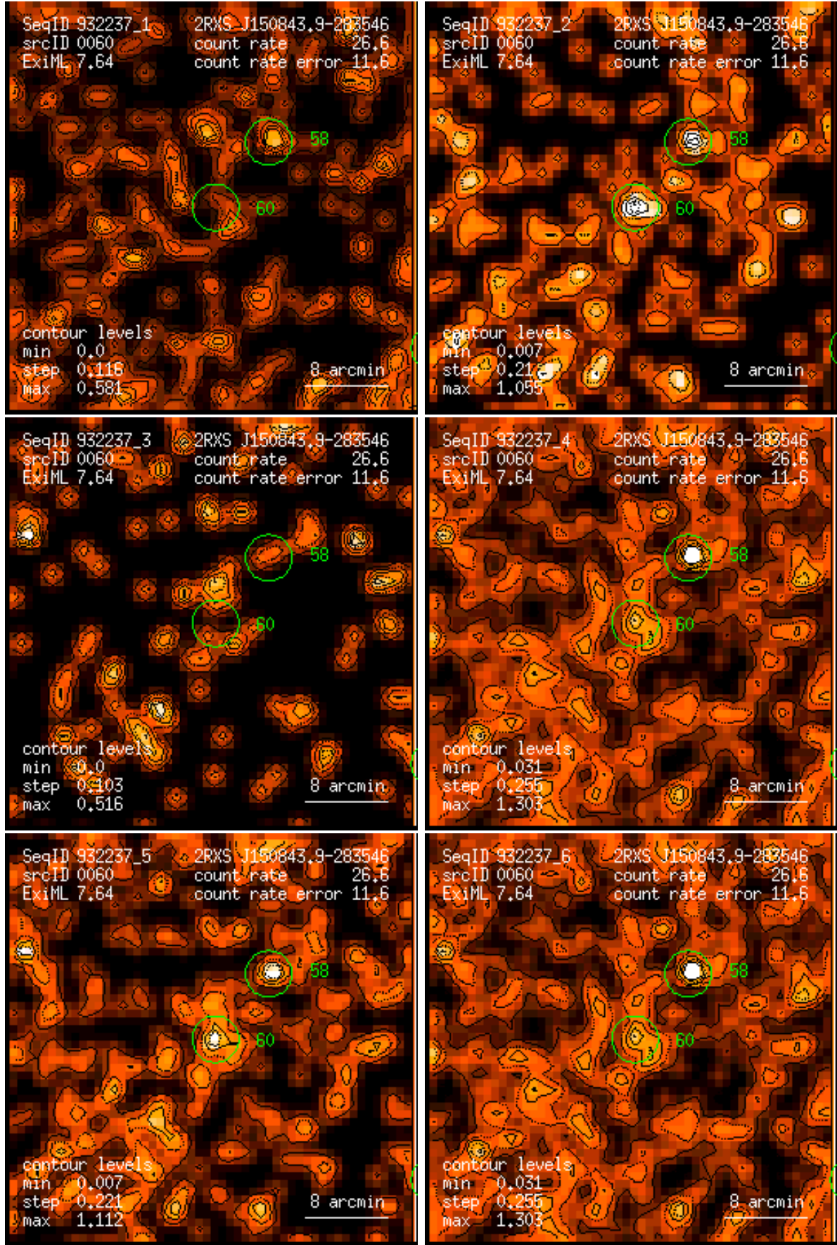
Figure 60: RASS 932237: detection 0060: band rate images, Gaussian filter: (1) PSPC channels 11 – 41, (2) 52 – 90, (3) 91 – 201, (4) 11 – 235, (5) 52 – 201, (6) 11 – 201. Broad band rates in counts/ks. Band rate contour levels in counts/ks/arcmin 2 .
