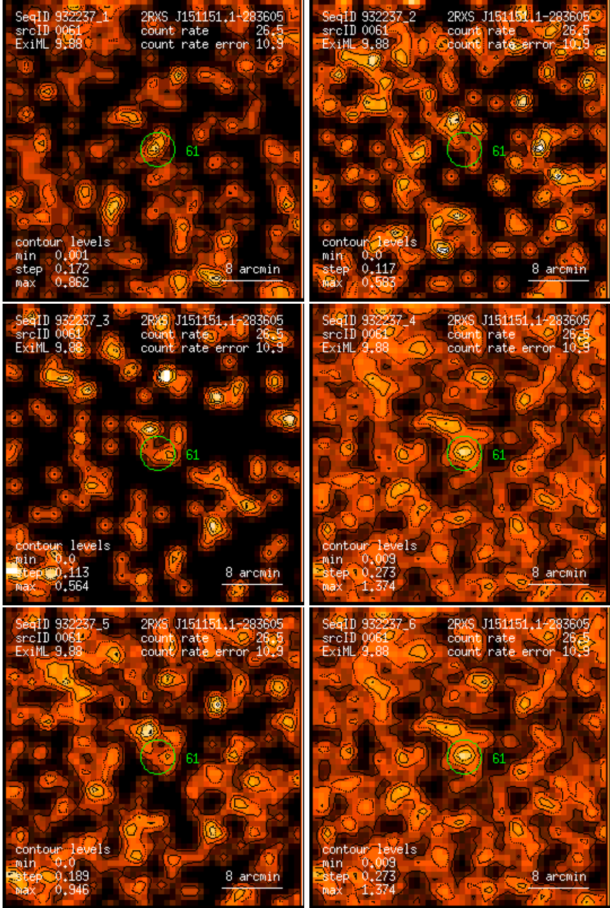
Figure 61: RASS 932237: detection 0061: band rate images, Gaussian filter: (1) PSPC channels 11 – 41, (2) 52 – 90, (3) 91 – 201, (4) 11 – 235, (5) 52 – 201, (6) 11 – 201. Broad band rates in counts/ks. Band rate contour levels in counts/ks/arcmin 2 .
