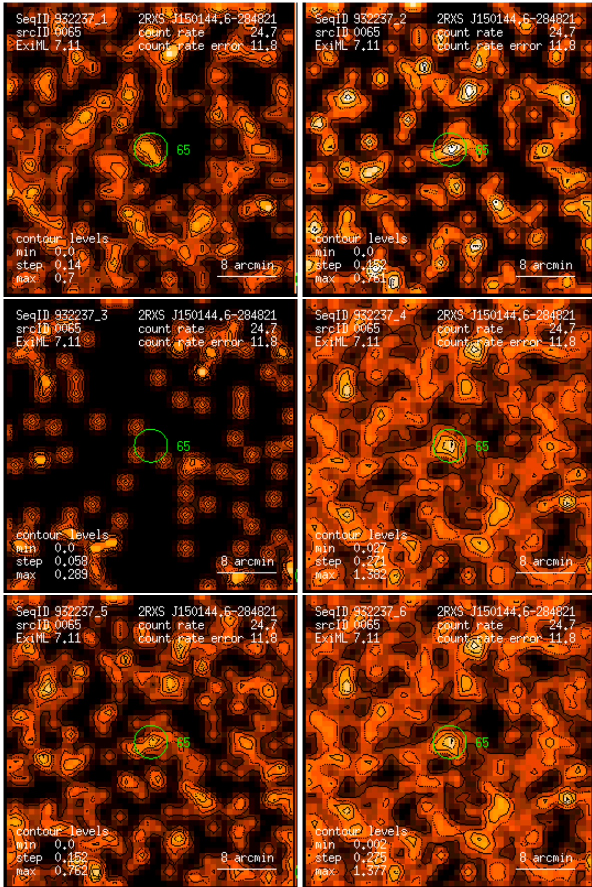
Figure 65: RASS 932237: detection 0065: band rate images, Gaussian filter: (1) PSPC channels 11 – 41, (2) 52 – 90, (3) 91 – 201, (4) 11 – 235, (5) 52 – 201, (6) 11 – 201. Broad band rates in counts/ks. Band rate contour levels in counts/ks/arcmin 2 .
