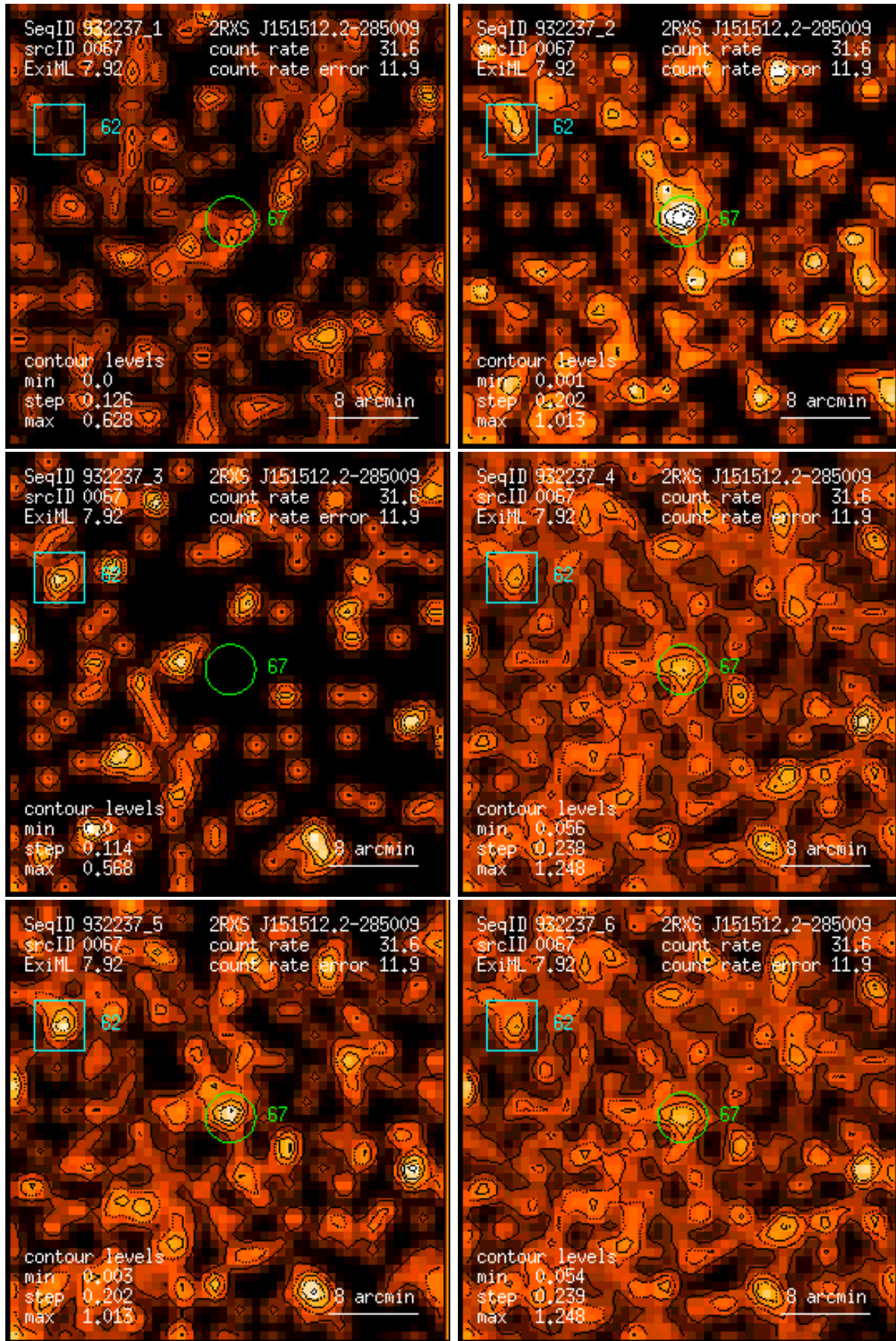
Figure 67: RASS 932237: detection 0067: band rate images, Gaussian filter: (1) PSPC channels 11 – 41, (2) 52 – 90, (3) 91 – 201, (4) 11 – 235, (5) 52 – 201, (6) 11 – 201. Broad band rates in counts/ks. Band rate contour levels in counts/ks/arcmin 2 .
