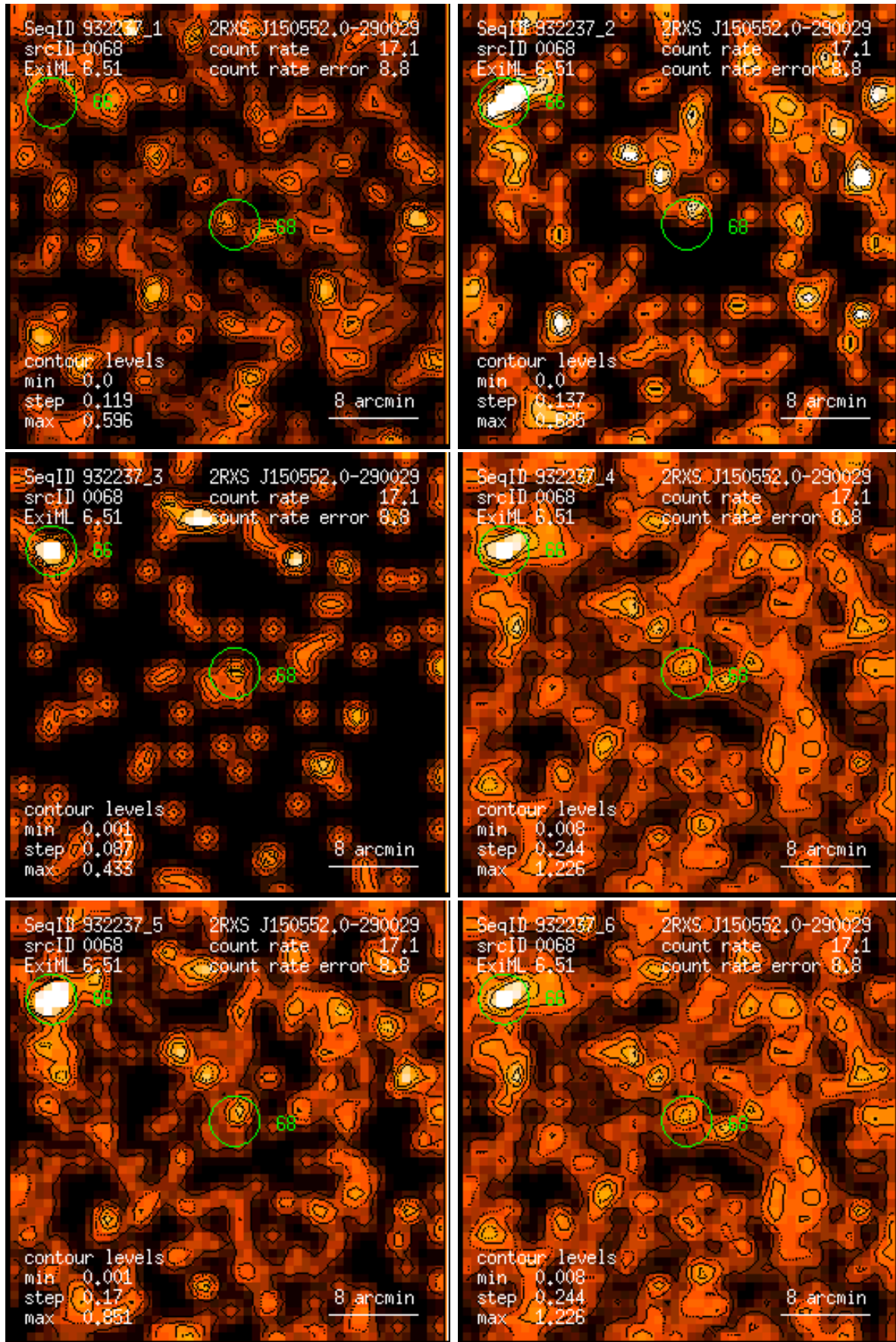
Figure 68: RASS 932237: detection 0068: band rate images, Gaussian filter: (1) PSPC channels 11 – 41, (2) 52 – 90, (3) 91 – 201, (4) 11 – 235, (5) 52 – 201, (6) 11 – 201. Broad band rates in counts/ks. Band rate contour levels in counts/ks/arcmin 2 .
