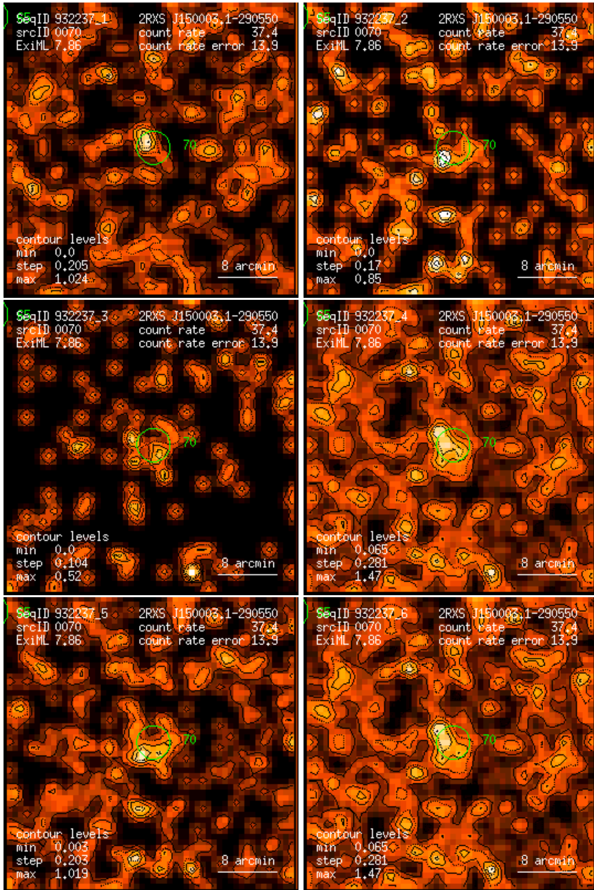
Figure 70: RASS 932237: detection 0070: band rate images, Gaussian filter: (1) PSPC channels 11 – 41, (2) 52 – 90, (3) 91 – 201, (4) 11 – 235, (5) 52 – 201, (6) 11 – 201. Broad band rates in counts/ks. Band rate contour levels in counts/ks/arcmin 2 .
