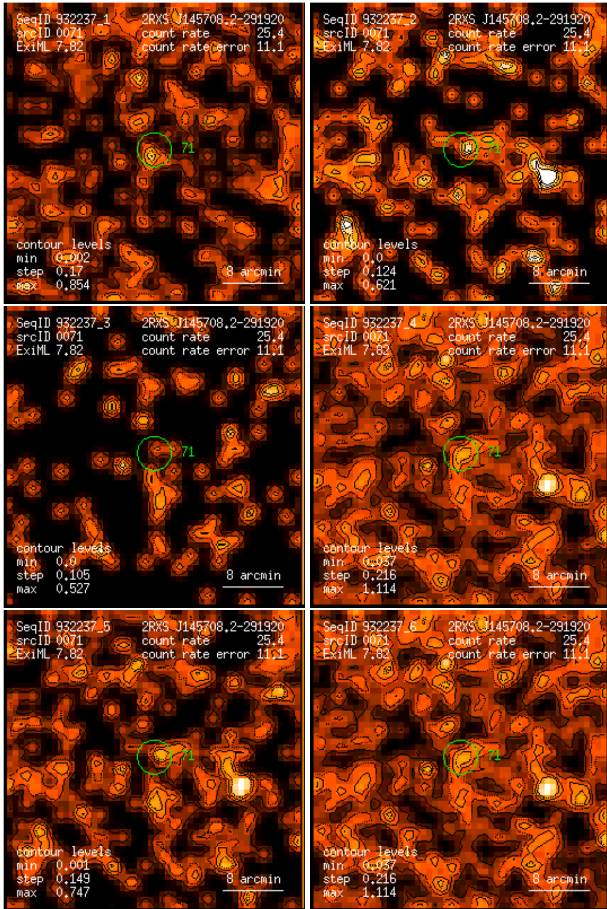
Figure 71: RASS 932237: detection 0071: band rate images, Gaussian filter: (1) PSPC channels 11 – 41, (2) 52 – 90, (3) 91 – 201, (4) 11 – 235, (5) 52 – 201, (6) 11 – 201. Broad band rates in counts/ks. Band rate contour levels in counts/ks/arcmin 2 .
