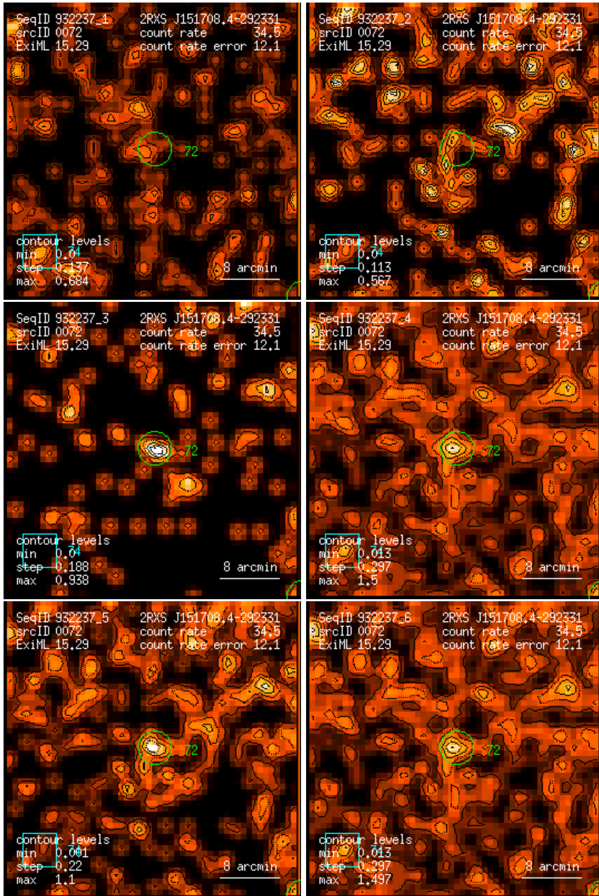
Figure 72: RASS 932237: detection 0072: band rate images, Gaussian filter: (1) PSPC channels 11 – 41, (2) 52 – 90, (3) 91 – 201, (4) 11 – 235, (5) 52 – 201, (6) 11 – 201. Broad band rates in counts/ks. Band rate contour levels in counts/ks/arcmin 2 .
