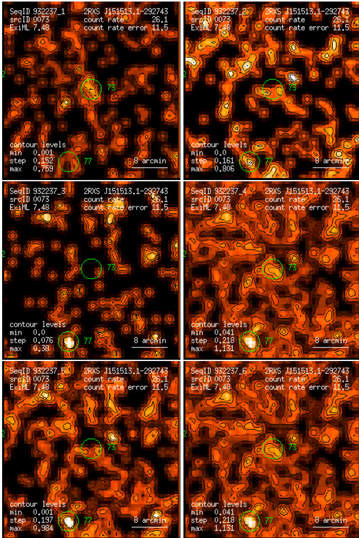
Figure 73: RASS 932237: detection 0073: band rate images, Gaussian filter: (1) PSPC channels 11 – 41, (2) 52 – 90, (3) 91 – 201, (4) 11 – 235, (5) 52 – 201, (6) 11 – 201. Broad band rates in counts/ks. Band rate contour levels in counts/ks/arcmin 2 .
