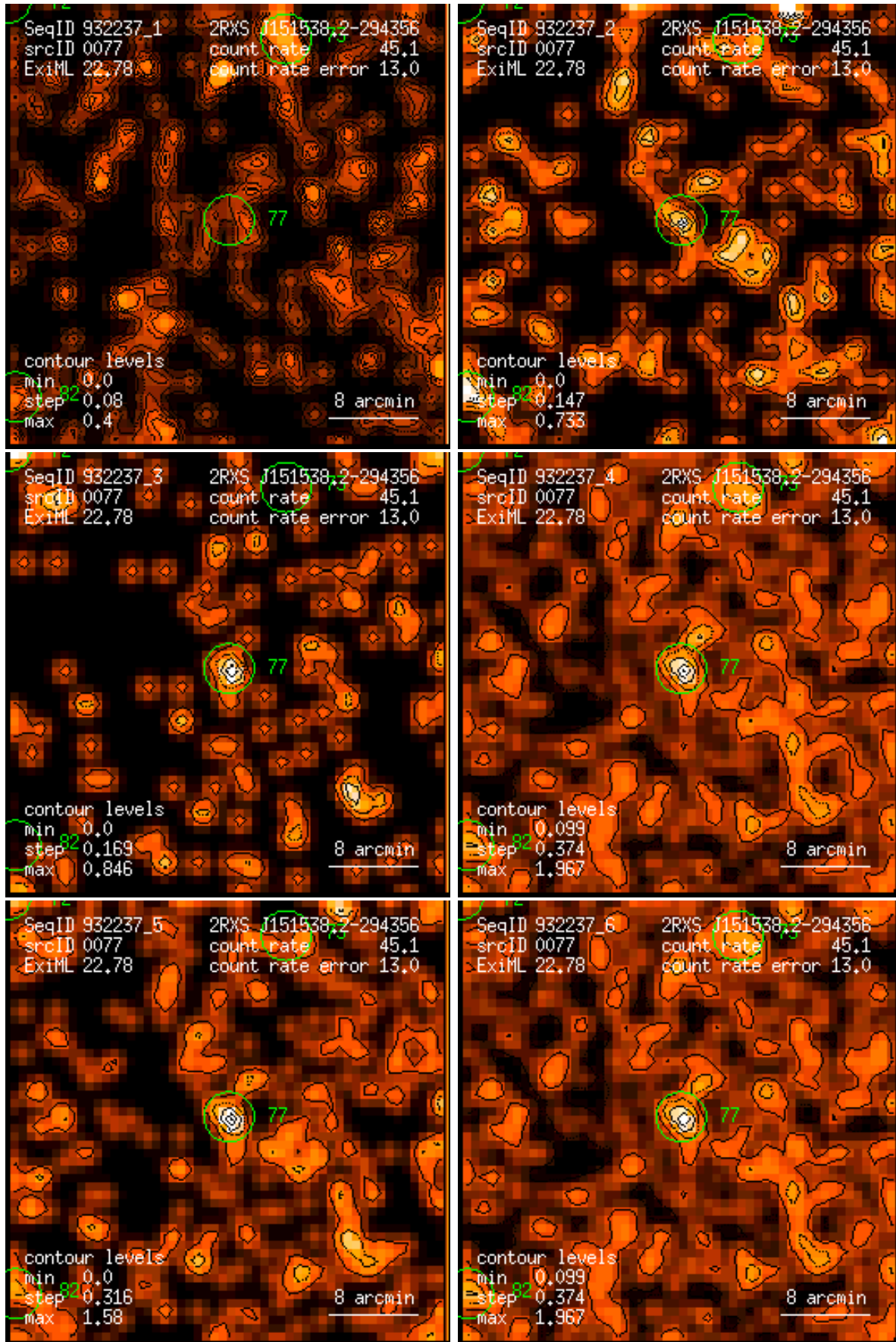
Figure 77: RASS 932237: detection 0077: band rate images, Gaussian filter: (1) PSPC channels 11 – 41, (2) 52 – 90, (3) 91 – 201, (4) 11 – 235, (5) 52 – 201, (6) 11 – 201. Broad band rates in counts/ks. Band rate contour levels in counts/ks/arcmin 2 .
