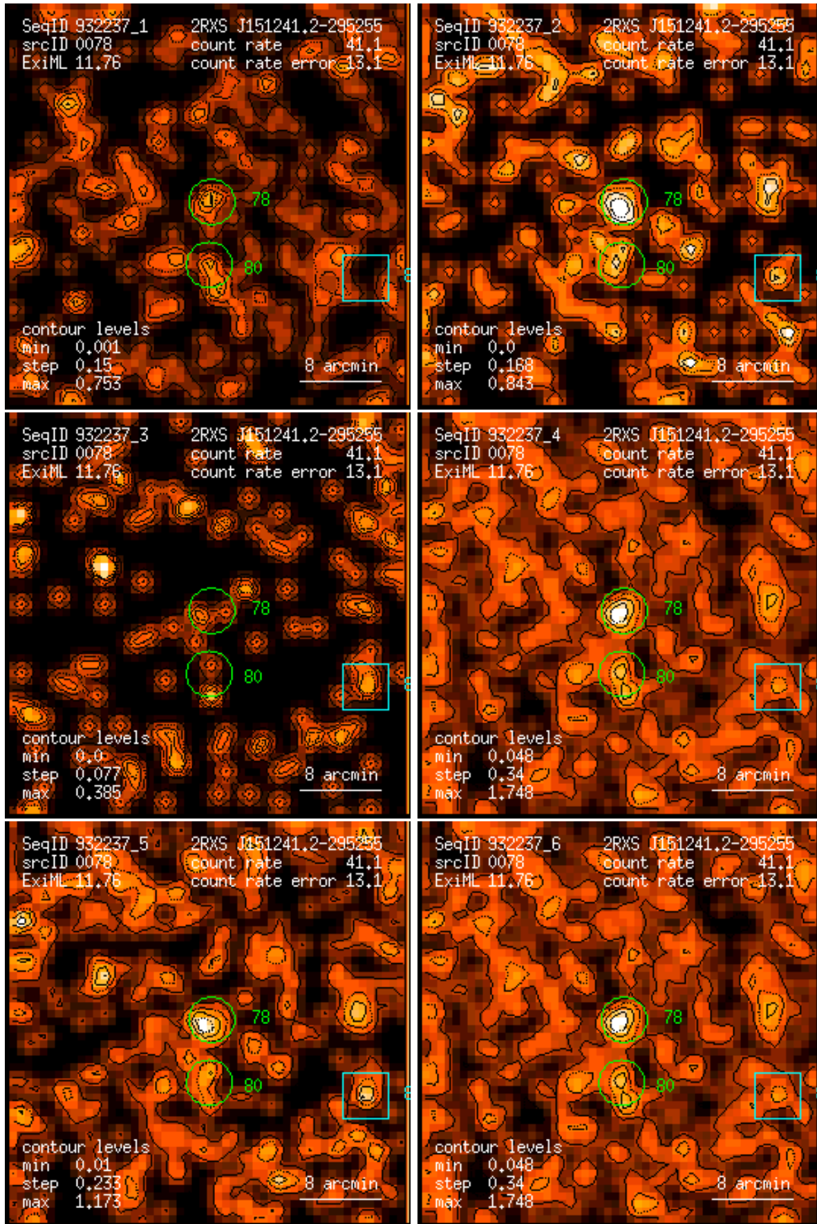
Figure 78: RASS 932237: detection 0078: band rate images, Gaussian filter: (1) PSPC channels 11 – 41, (2) 52 – 90, (3) 91 – 201, (4) 11 – 235, (5) 52 – 201, (6) 11 – 201. Broad band rates in counts/ks. Band rate contour levels in counts/ks/arcmin 2 .
