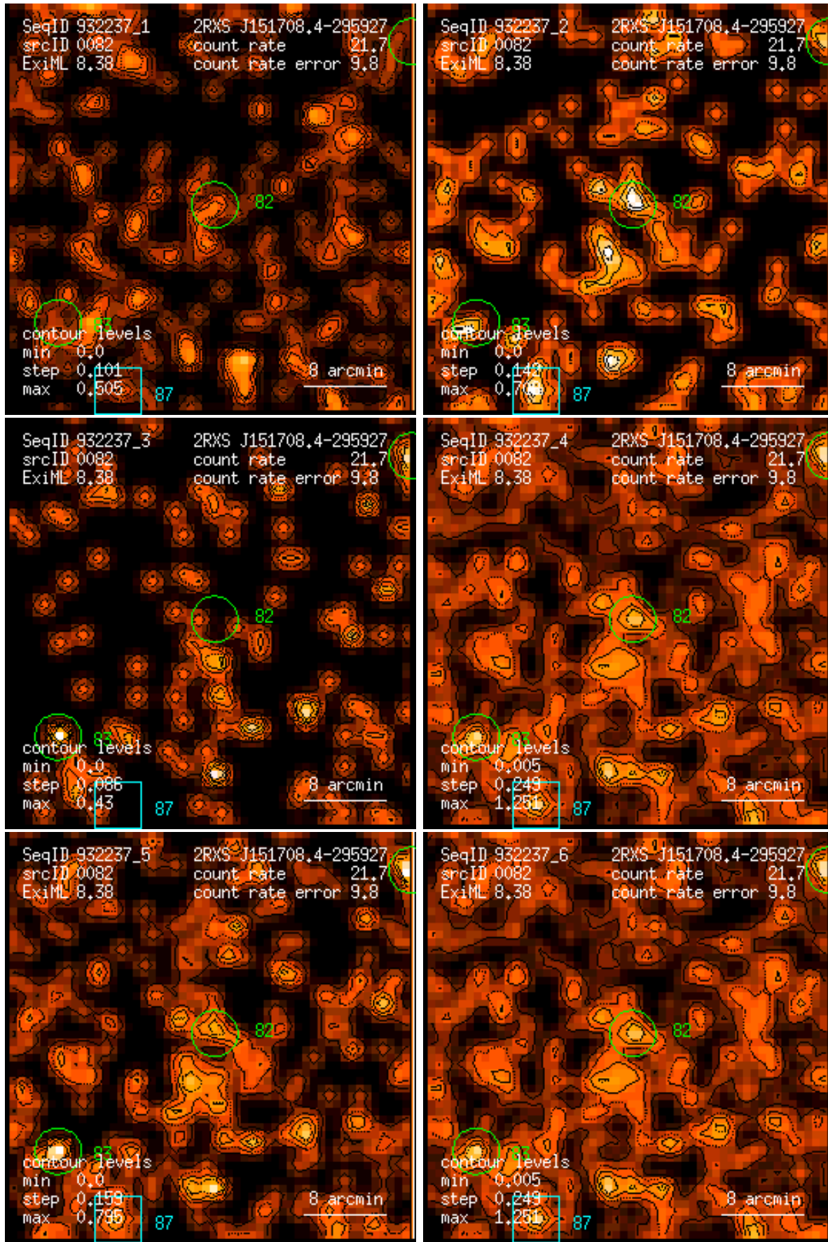
Figure 82: RASS 932237: detection 0082: band rate images, Gaussian filter: (1) PSPC channels 11 – 41, (2) 52 – 90, (3) 91 – 201, (4) 11 – 235, (5) 52 – 201, (6) 11 – 201. Broad band rates in counts/ks. Band rate contour levels in counts/ks/arcmin 2 .
