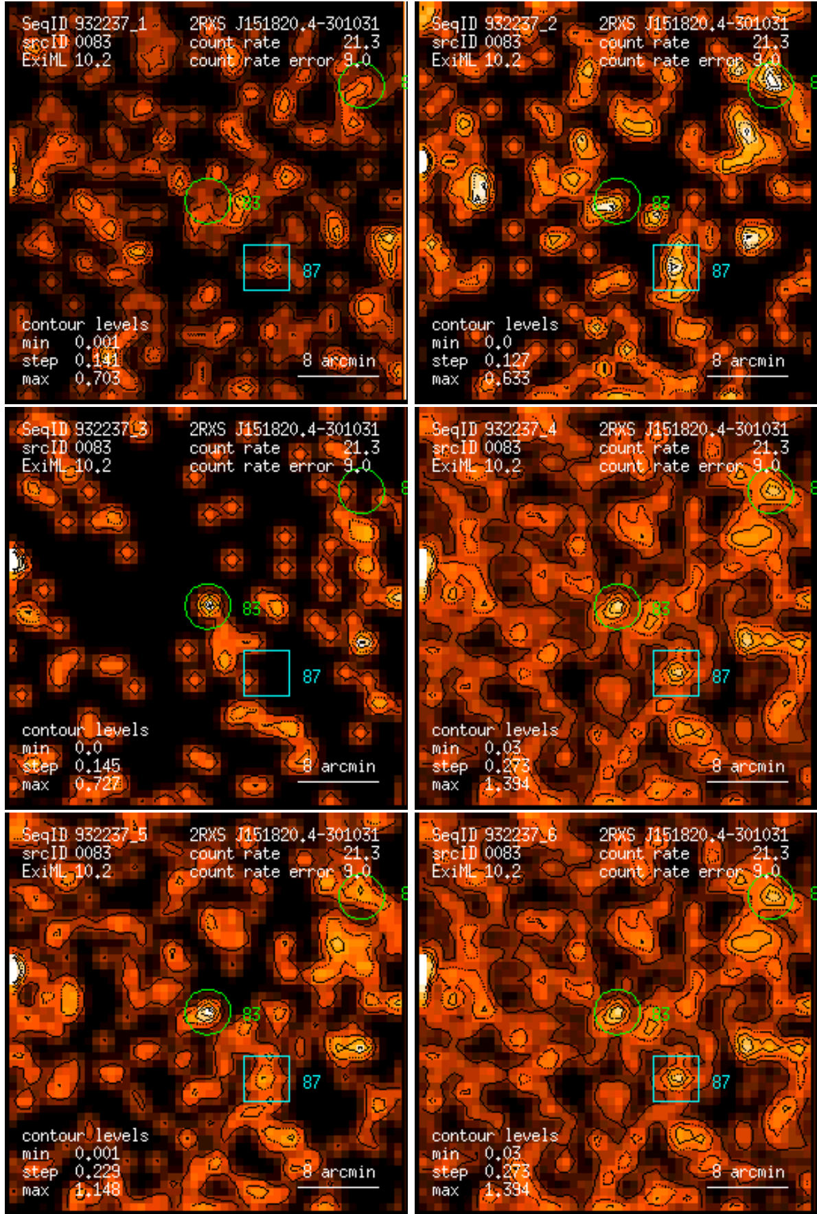
Figure 83: RASS 932237: detection 0083: band rate images, Gaussian filter: (1) PSPC channels 11 – 41, (2) 52 – 90, (3) 91 – 201, (4) 11 – 235, (5) 52 – 201, (6) 11 – 201. Broad band rates in counts/ks. Band rate contour levels in counts/ks/arcmin 2 .
