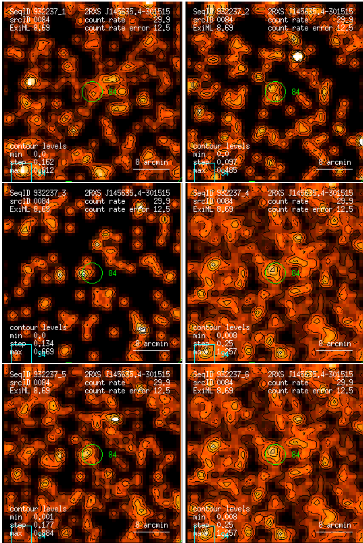
Figure 84: RASS 932237: detection 0084: band rate images, Gaussian filter: (1) PSPC channels 11 – 41, (2) 52 – 90, (3) 91 – 201, (4) 11 – 235, (5) 52 – 201, (6) 11 – 201. Broad band rates in counts/ks. Band rate contour levels in counts/ks/arcmin 2 .
