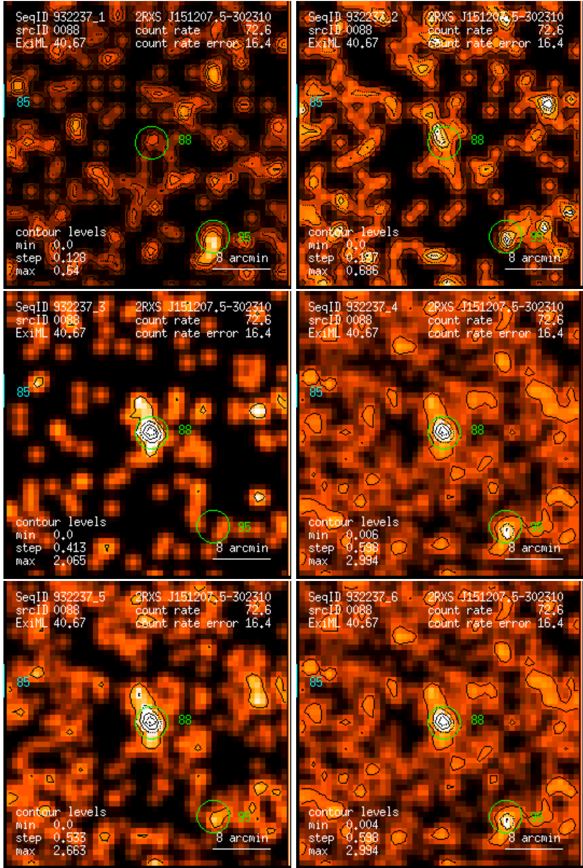
Figure 88: RASS 932237: detection 0088: band rate images, Gaussian filter: (1) PSPC channels 11 – 41, (2) 52 – 90, (3) 91 – 201, (4) 11 – 235, (5) 52 – 201, (6) 11 – 201. Broad band rates in counts/ks. Band rate contour levels in counts/ks/arcmin 2 .
