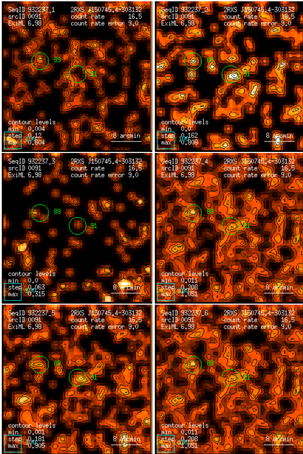
Figure 91: RASS 932237: detection 0091: band rate images, Gaussian filter: (1) PSPC channels 11 – 41, (2) 52 – 90, (3) 91 – 201, (4) 11 – 235, (5) 52 – 201, (6) 11 – 201. Broad band rates in counts/ks. Band rate contour levels in counts/ks/arcmin 2 .
