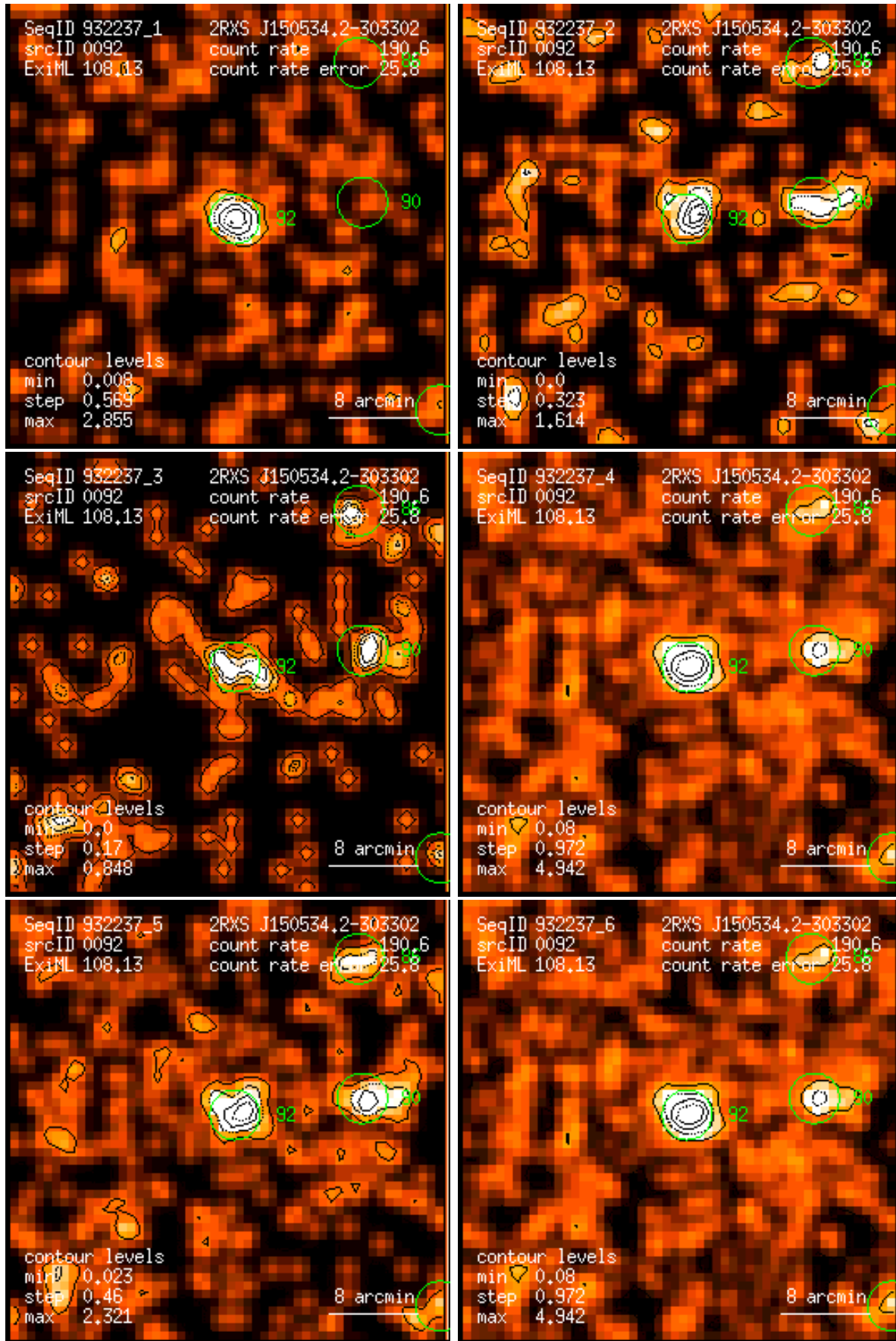
Figure 92: RASS 932237: detection 0092: band rate images, Gaussian filter: (1) PSPC channels 11 – 41, (2) 52 – 90, (3) 91 – 201, (4) 11 – 235, (5) 52 – 201, (6) 11 – 201. Broad band rates in counts/ks. Band rate contour levels in counts/ks/arcmin 2 .
