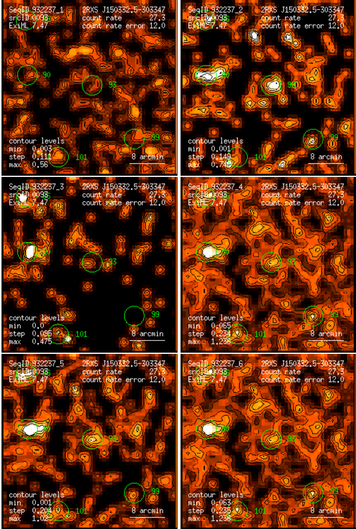
Figure 93: RASS 932237: detection 0093: band rate images, Gaussian filter: (1) PSPC channels 11 – 41, (2) 52 – 90, (3) 91 – 201, (4) 11 – 235, (5) 52 – 201, (6) 11 – 201. Broad band rates in counts/ks. Band rate contour levels in counts/ks/arcmin 2 .
