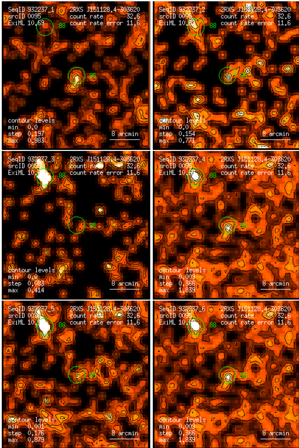
Figure 95: RASS 932237: detection 0095: band rate images, Gaussian filter: (1) PSPC channels 11 – 41, (2) 52 – 90, (3) 91 – 201, (4) 11 – 235, (5) 52 – 201, (6) 11 – 201. Broad band rates in counts/ks. Band rate contour levels in counts/ks/arcmin 2 .
