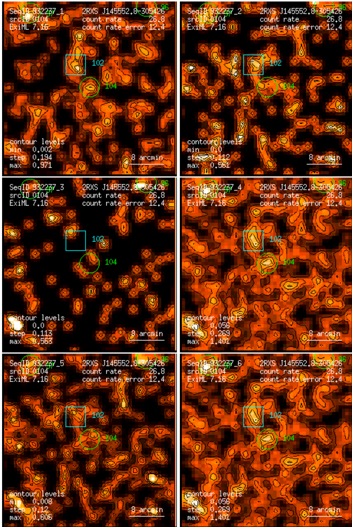
Figure 104: RASS 932237: detection 0104: band rate images, Gaussian filter: (1) PSPC channels 11 – 41, (2) 52 – 90, (3) 91 – 201, (4) 11 – 235, (5) 52 – 201, (6) 11 – 201. Broad band rates in counts/ks. Band rate contour levels in counts/ks/arcmin 2 .
