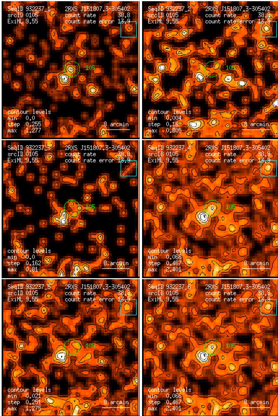
Figure 105: RASS 932237: detection 0105: band rate images, Gaussian filter: (1) PSPC channels 11 – 41, (2) 52 – 90, (3) 91 – 201, (4) 11 – 235, (5) 52 – 201, (6) 11 – 201. Broad band rates in counts/ks. Band rate contour levels in counts/ks/arcmin 2 .
