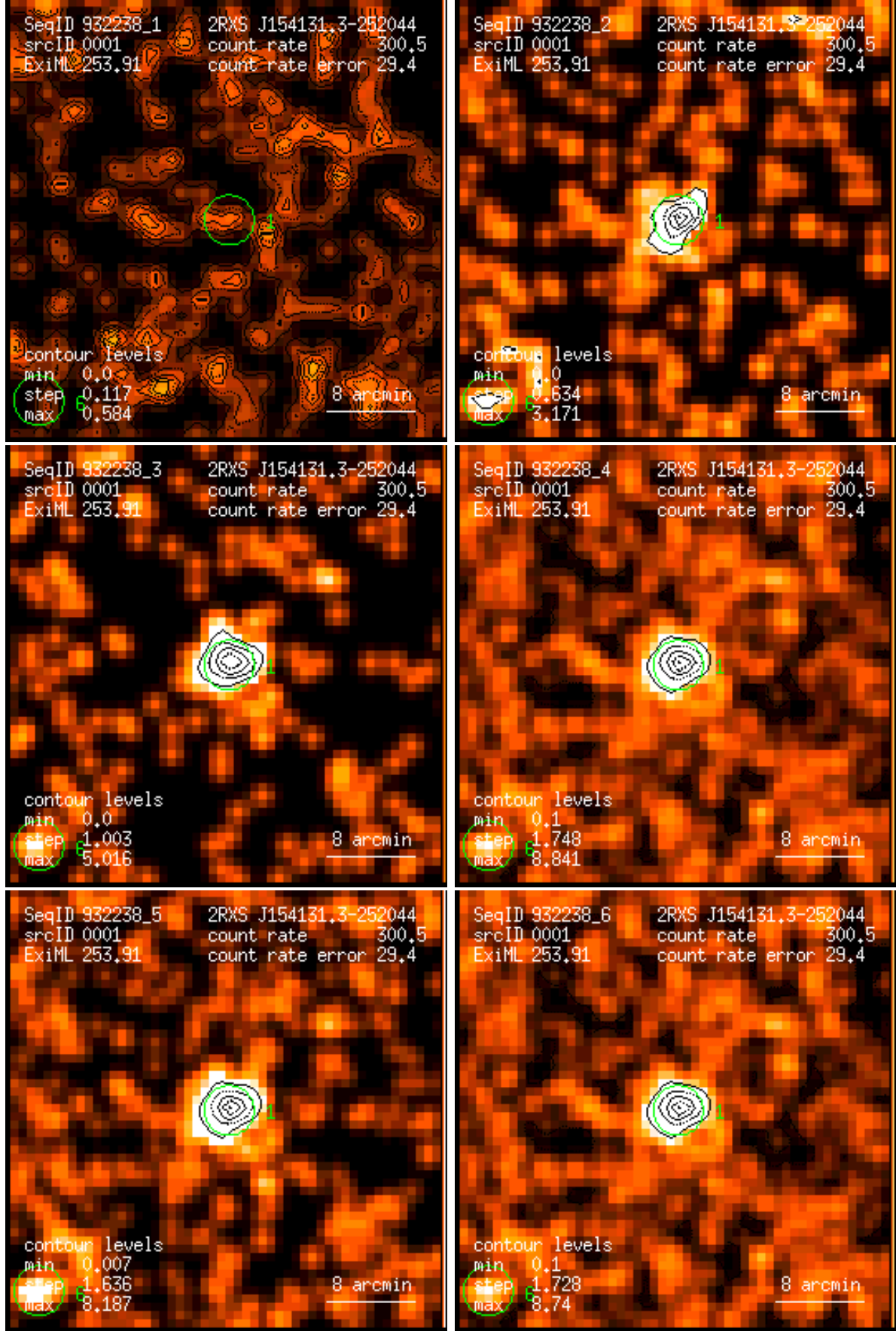
Figure 1: RASS 932238: detection 0001: band rate images, Gaussian filter: (1) PSPC channels 11 – 41, (2) 52 – 90, (3) 91 – 201, (4) 11 – 235, (5) 52 – 201, (6) 11 – 201. Broad band rates in counts/ks. Band rate contour levels in counts/ks/arcmin 2 .
