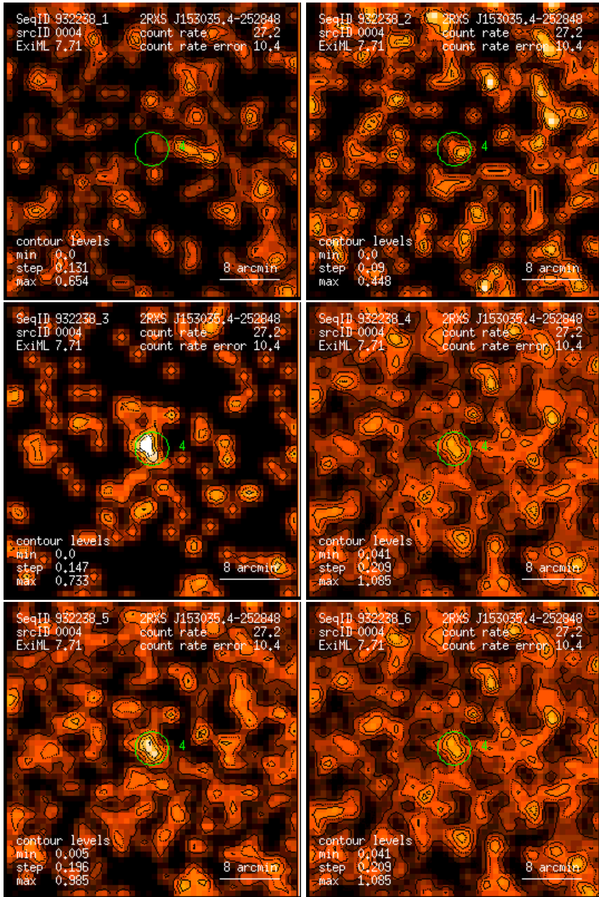
Figure 4: RASS 932238: detection 0004: band rate images, Gaussian filter: (1) PSPC channels 11 – 41, (2) 52 – 90, (3) 91 – 201, (4) 11 – 235, (5) 52 – 201, (6) 11 – 201. Broad band rates in counts/ks. Band rate contour levels in counts/ks/arcmin 2 .
