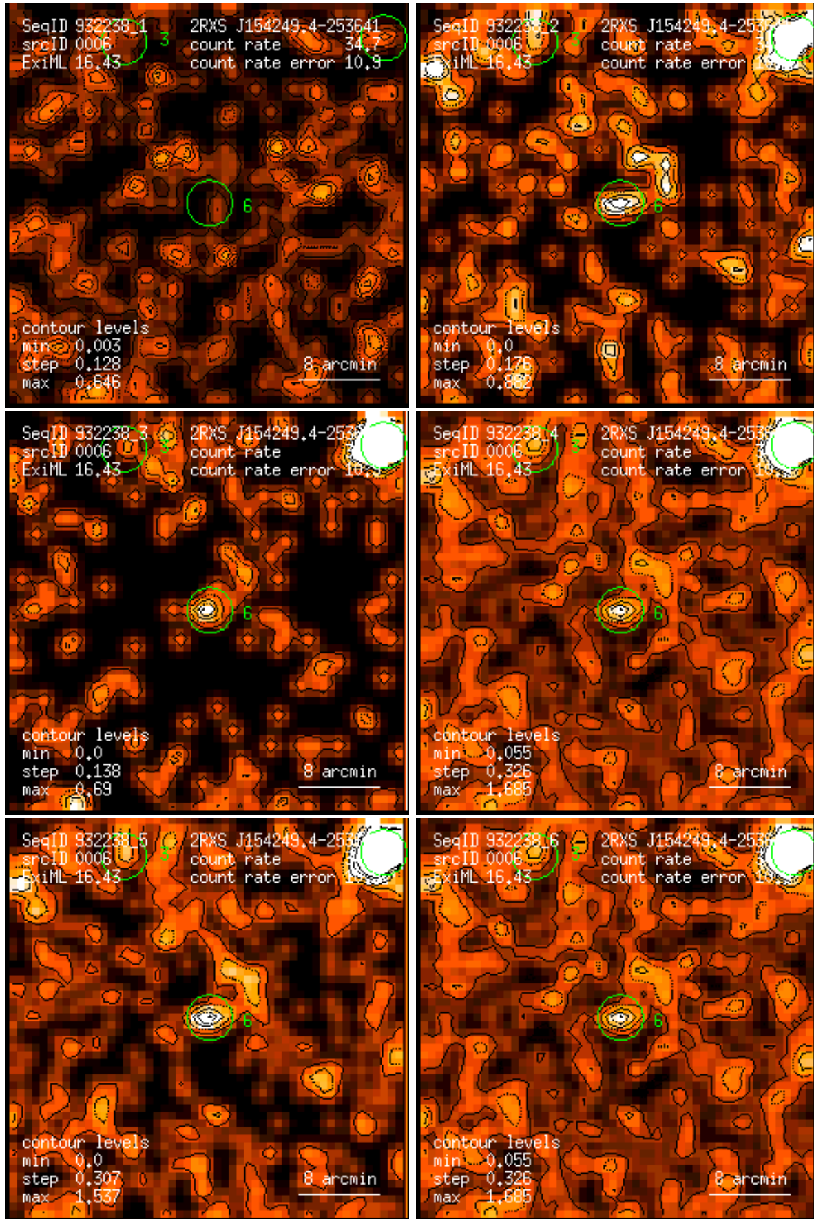
Figure 6: RASS 932238: detection 0006: band rate images, Gaussian filter: (1) PSPC channels 11 – 41, (2) 52 – 90, (3) 91 – 201, (4) 11 – 235, (5) 52 – 201, (6) 11 – 201. Broad band rates in counts/ks. Band rate contour levels in counts/ks/arcmin 2 .
