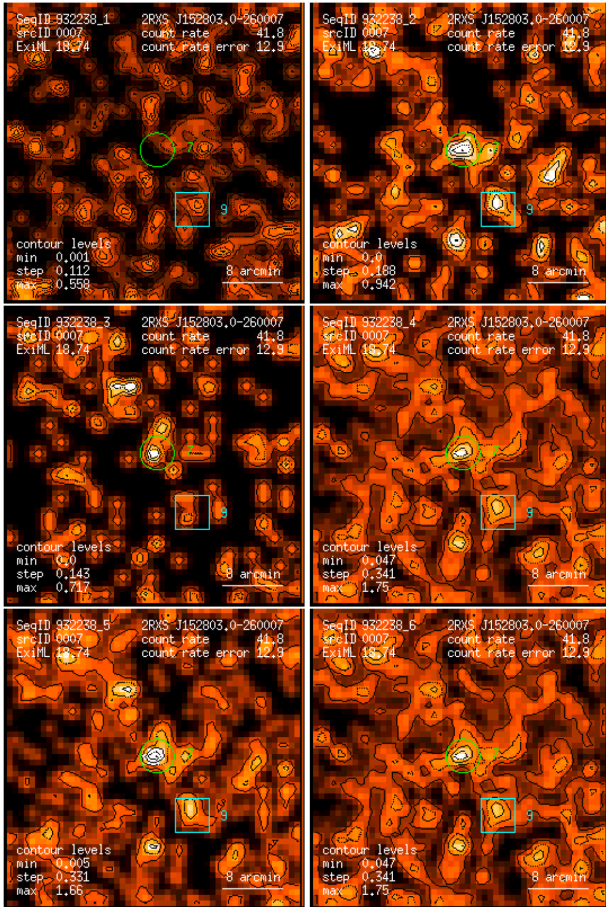
Figure 7: RASS 932238: detection 0007: band rate images, Gaussian filter: (1) PSPC channels 11 – 41, (2) 52 – 90, (3) 91 – 201, (4) 11 – 235, (5) 52 – 201, (6) 11 – 201. Broad band rates in counts/ks. Band rate contour levels in counts/ks/arcmin 2 .
