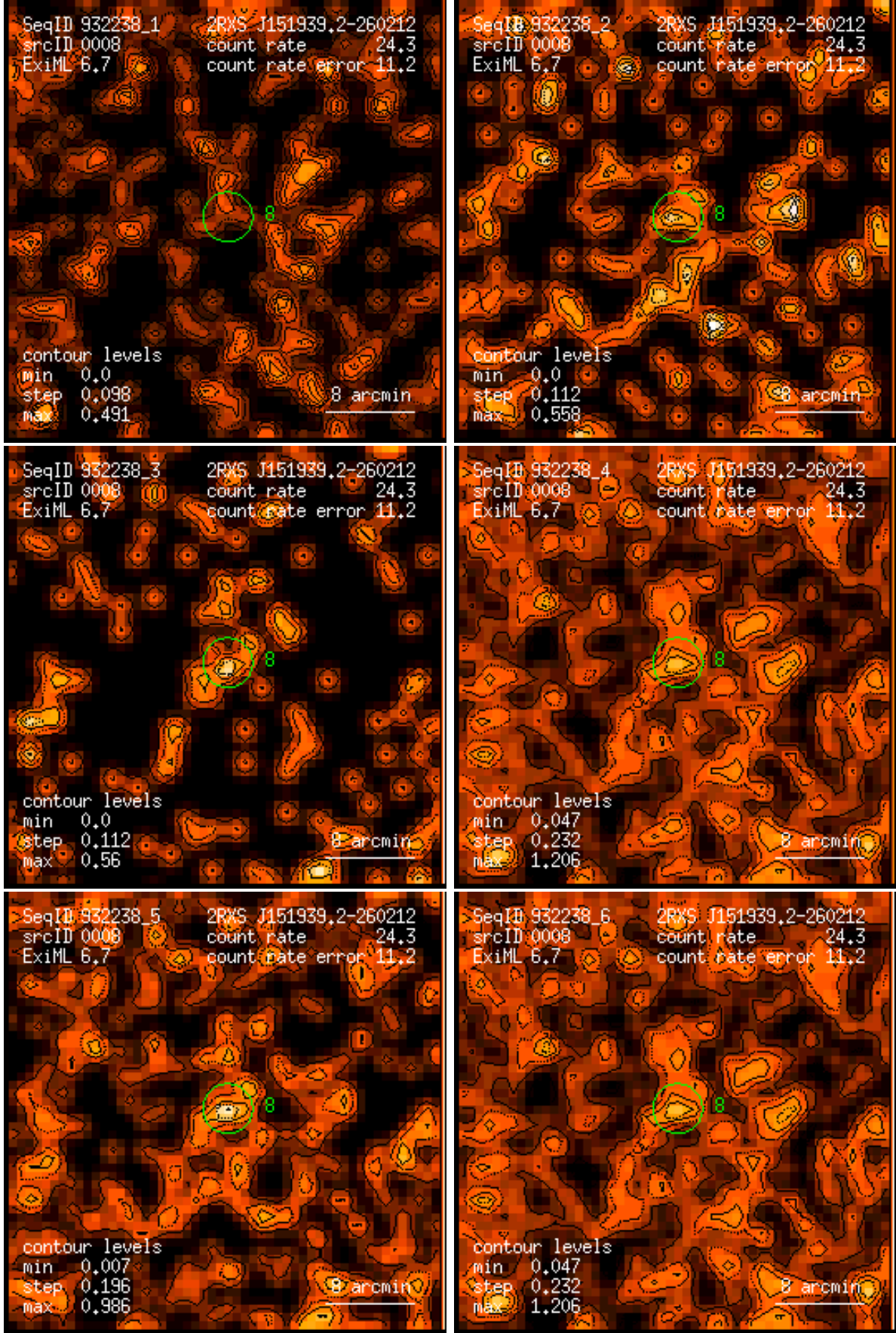
Figure 8: RASS 932238: detection 0008: band rate images, Gaussian filter: (1) PSPC channels 11 – 41, (2) 52 – 90, (3) 91 – 201, (4) 11 – 235, (5) 52 – 201, (6) 11 – 201. Broad band rates in counts/ks. Band rate contour levels in counts/ks/arcmin 2 .
