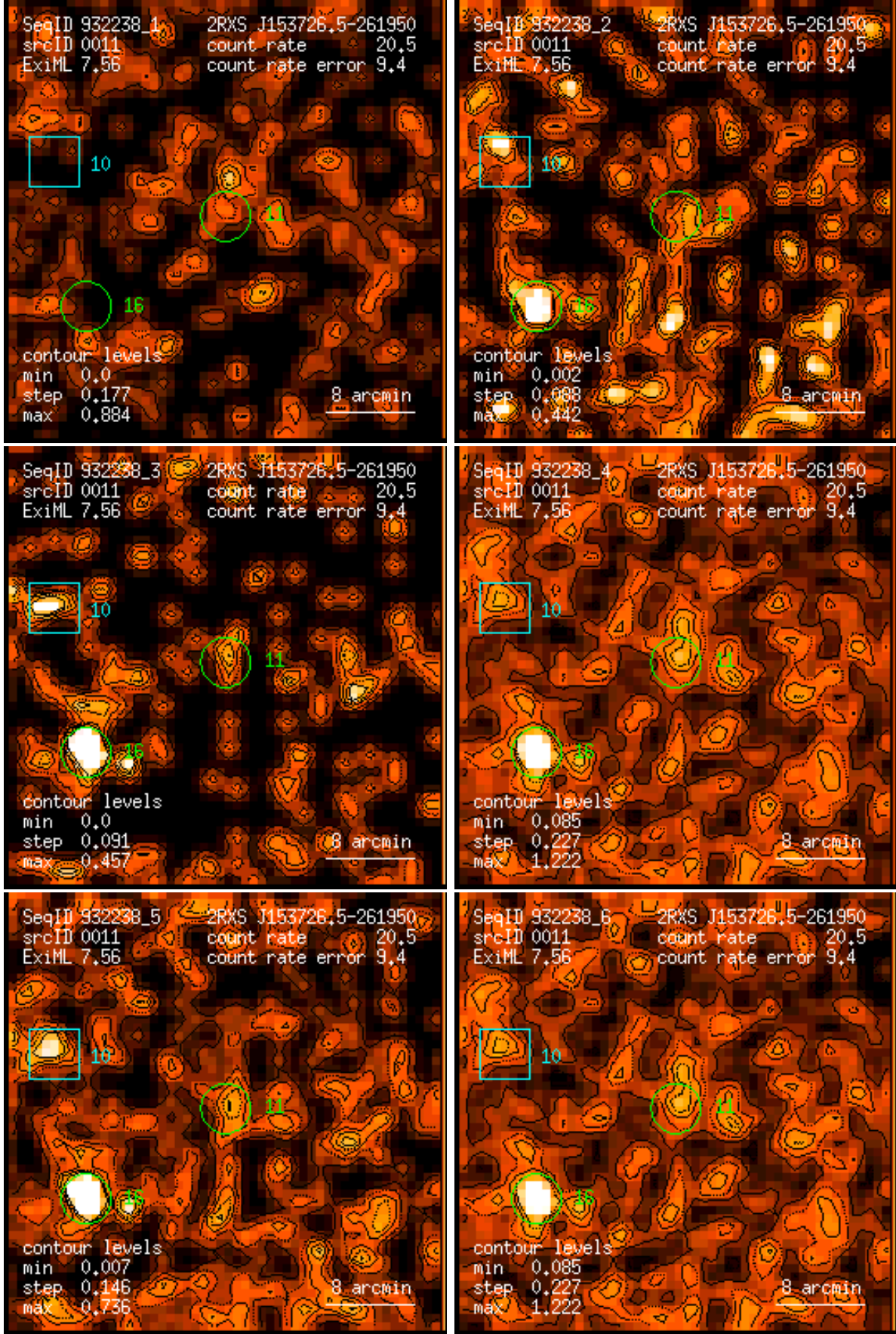
Figure 11: RASS 932238: detection 0011: band rate images, Gaussian filter: (1) PSPC channels 11 – 41, (2) 52 – 90, (3) 91 – 201, (4) 11 – 235, (5) 52 – 201, (6) 11 – 201. Broad band rates in counts/ks. Band rate contour levels in counts/ks/arcmin 2 .
