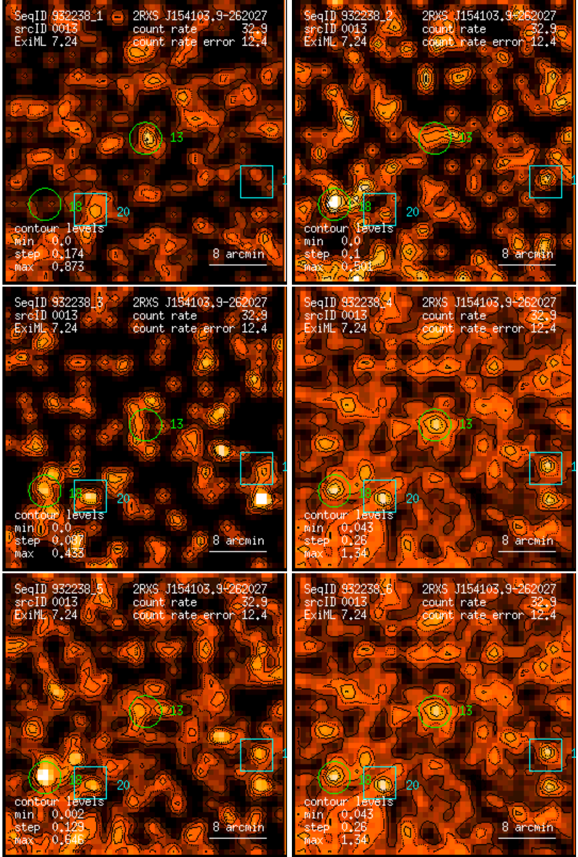
Figure 13: RASS 932238: detection 0013: band rate images, Gaussian filter: (1) PSPC channels 11 – 41, (2) 52 – 90, (3) 91 – 201, (4) 11 – 235, (5) 52 – 201, (6) 11 – 201. Broad band rates in counts/ks. Band rate contour levels in counts/ks/arcmin 2 .
