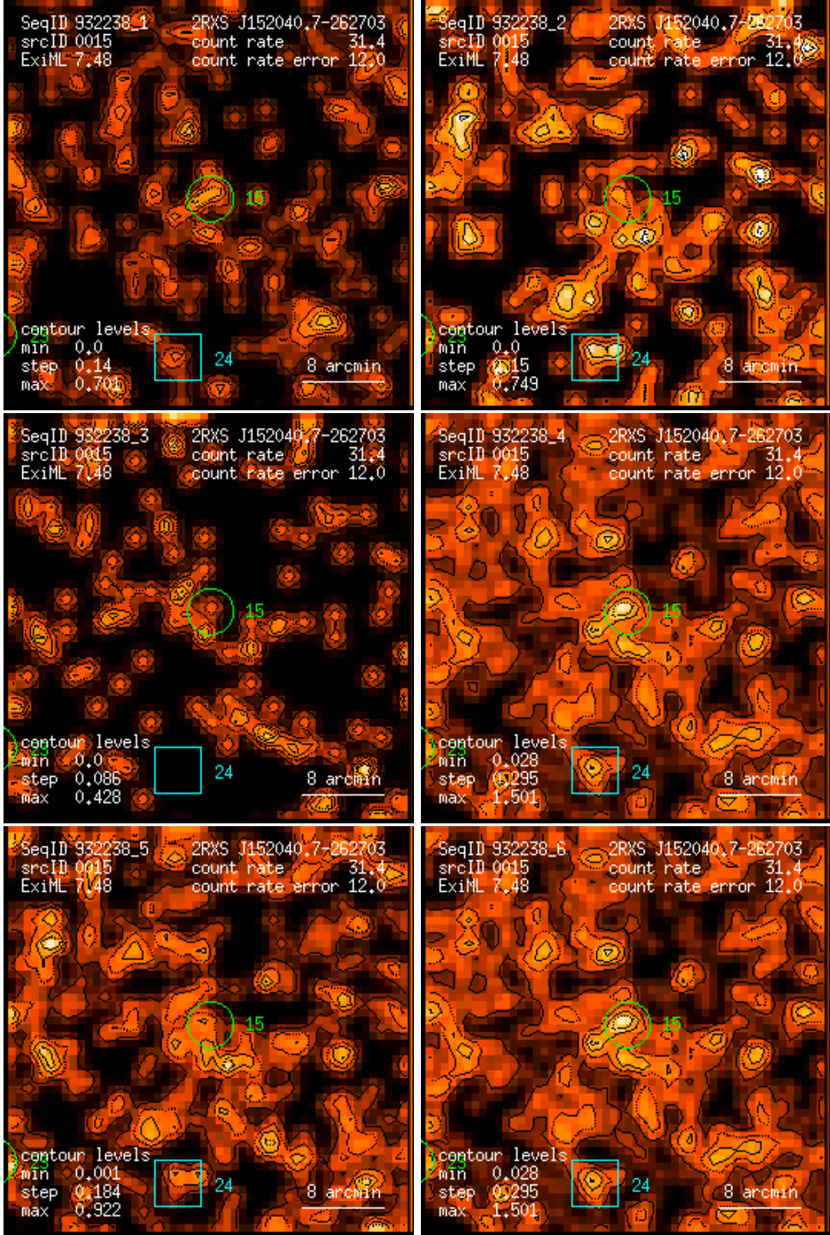
Figure 15: RASS 932238: detection 0015: band rate images, Gaussian filter: (1) PSPC channels 11 – 41, (2) 52 – 90, (3) 91 – 201, (4) 11 – 235, (5) 52 – 201, (6) 11 – 201. Broad band rates in counts/ks. Band rate contour levels in counts/ks/arcmin 2 .
