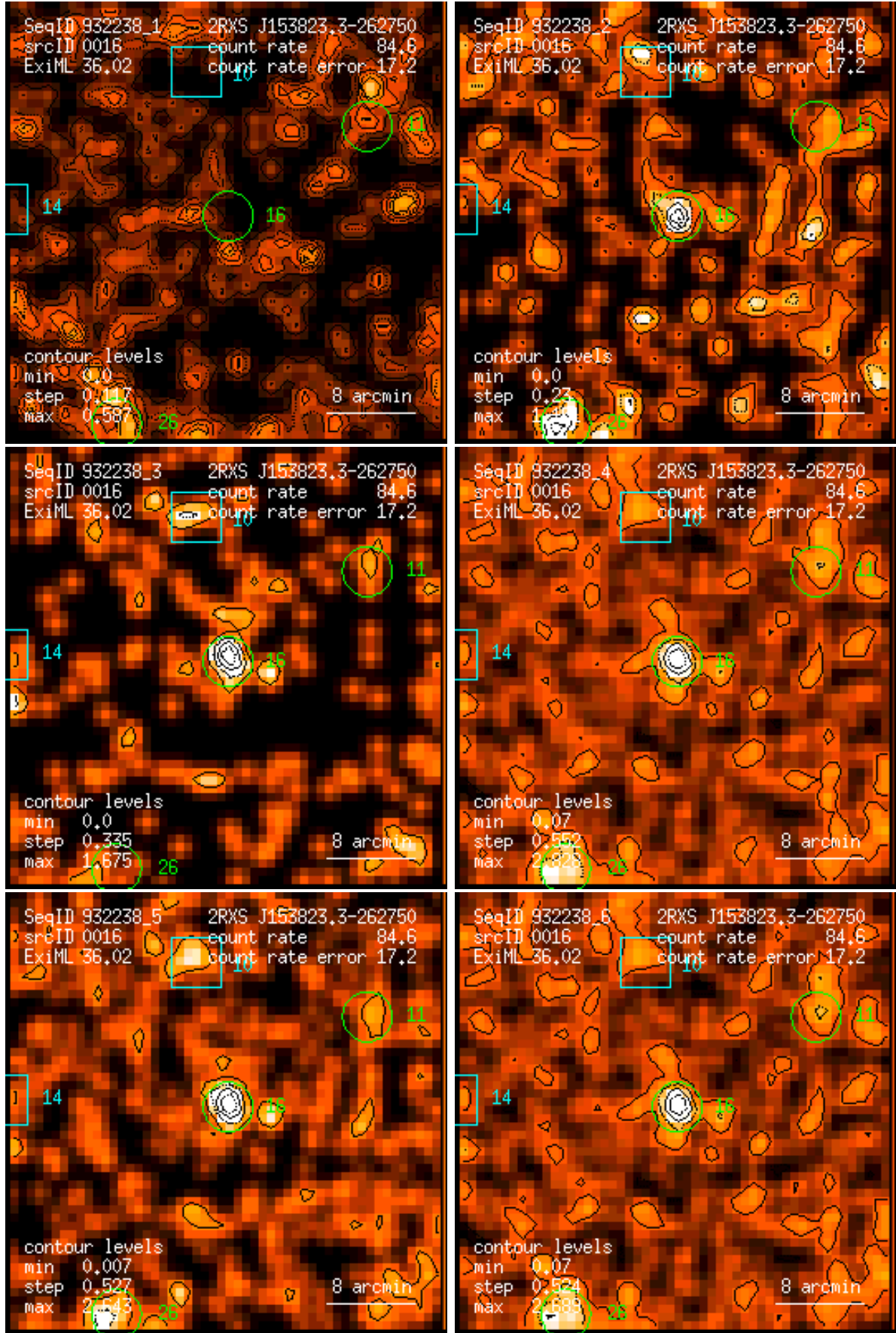
Figure 16: RASS 932238: detection 0016: band rate images, Gaussian filter: (1) PSPC channels 11 – 41, (2) 52 – 90, (3) 91 – 201, (4) 11 – 235, (5) 52 – 201, (6) 11 – 201. Broad band rates in counts/ks. Band rate contour levels in counts/ks/arcmin 2 .
