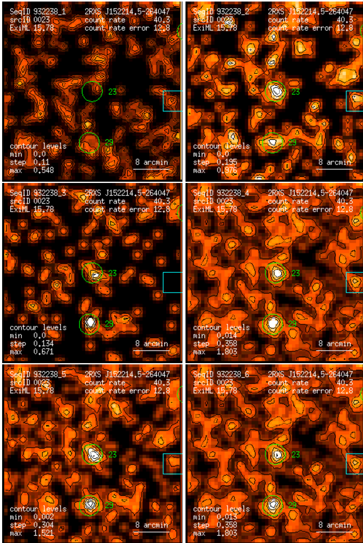
Figure 23: RASS 932238: detection 0023: band rate images, Gaussian filter: (1) PSPC channels 11 – 41, (2) 52 – 90, (3) 91 – 201, (4) 11 – 235, (5) 52 – 201, (6) 11 – 201. Broad band rates in counts/ks. Band rate contour levels in counts/ks/arcmin 2 .
