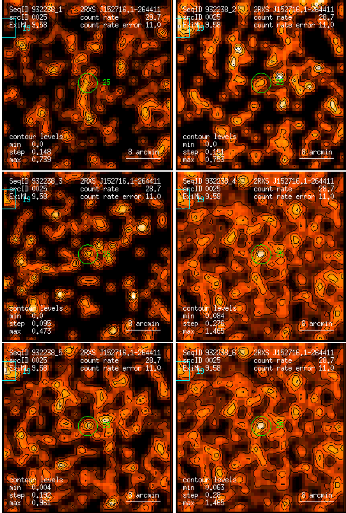
Figure 25: RASS 932238: detection 0025: band rate images, Gaussian filter: (1) PSPC channels 11 – 41, (2) 52 – 90, (3) 91 – 201, (4) 11 – 235, (5) 52 – 201, (6) 11 – 201. Broad band rates in counts/ks. Band rate contour levels in counts/ks/arcmin 2 .
