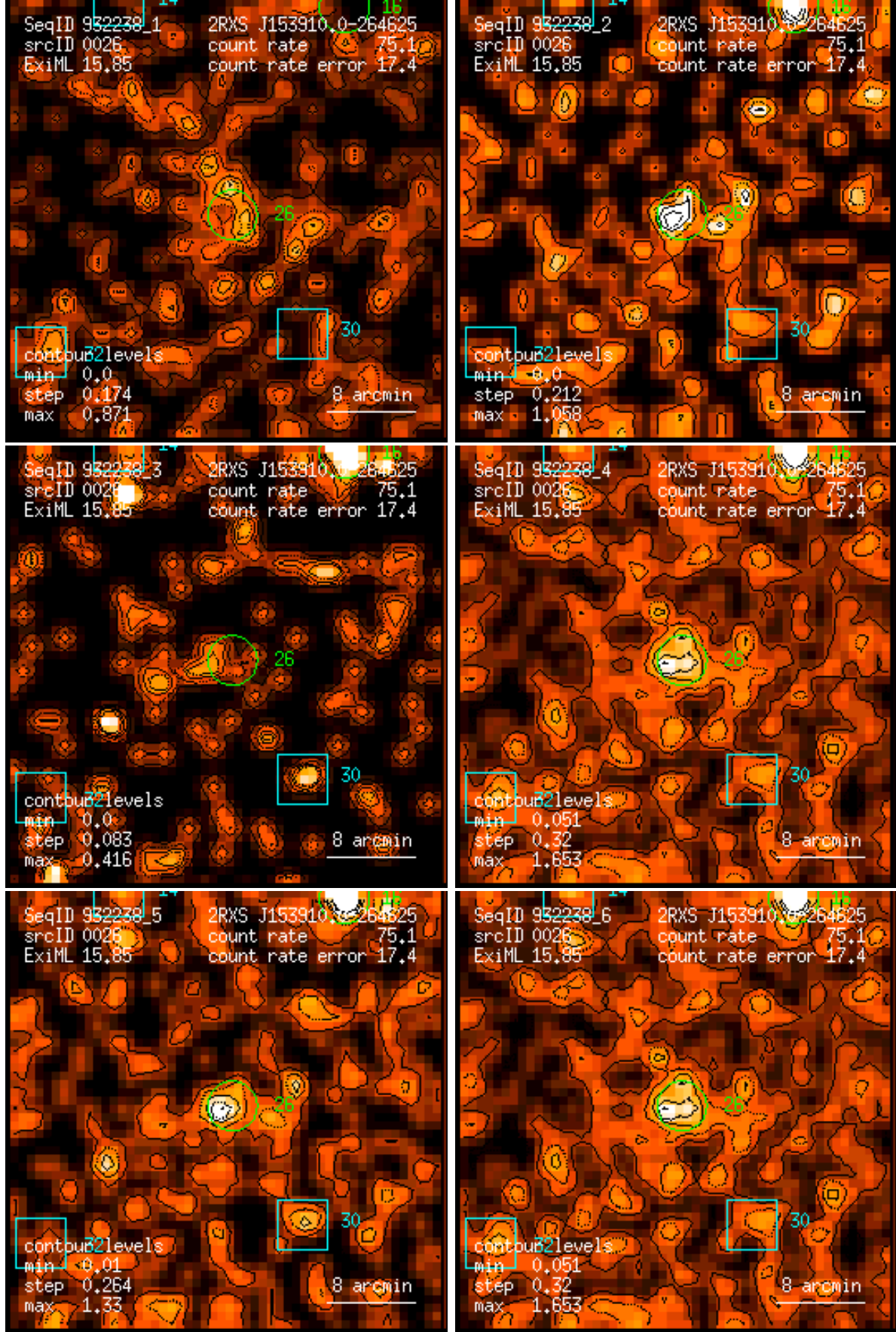
Figure 26: RASS 932238: detection 0026: band rate images, Gaussian filter: (1) PSPC channels 11 – 41, (2) 52 – 90, (3) 91 – 201, (4) 11 – 235, (5) 52 – 201, (6) 11 – 201. Broad band rates in counts/ks. Band rate contour levels in counts/ks/arcmin 2 .
