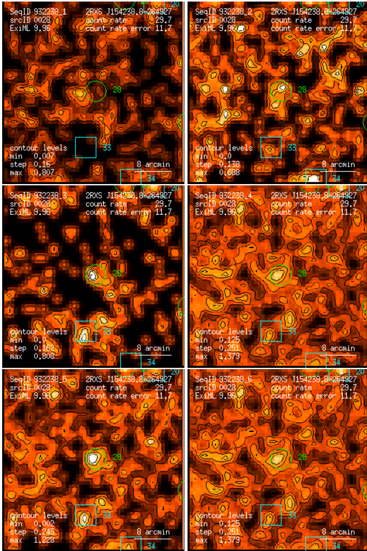
Figure 28: RASS 932238: detection 0028: band rate images, Gaussian filter: (1) PSPC channels 11 – 41, (2) 52 – 90, (3) 91 – 201, (4) 11 – 235, (5) 52 – 201, (6) 11 – 201. Broad band rates in counts/ks. Band rate contour levels in counts/ks/arcmin 2 .
