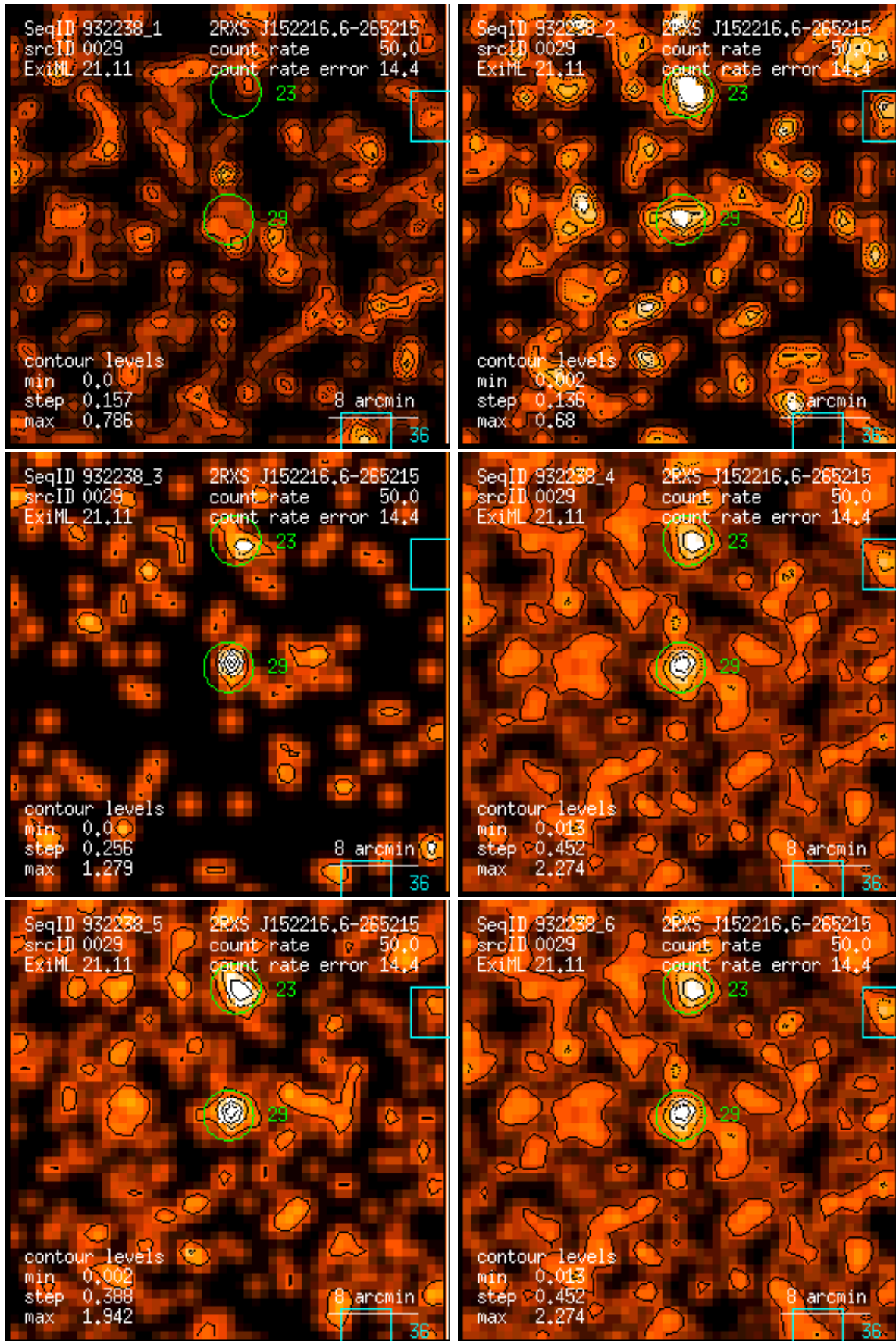
Figure 29: RASS 932238: detection 0029: band rate images, Gaussian filter: (1) PSPC channels 11 – 41, (2) 52 – 90, (3) 91 – 201, (4) 11 – 235, (5) 52 – 201, (6) 11 – 201. Broad band rates in counts/ks. Band rate contour levels in counts/ks/arcmin 2 .
