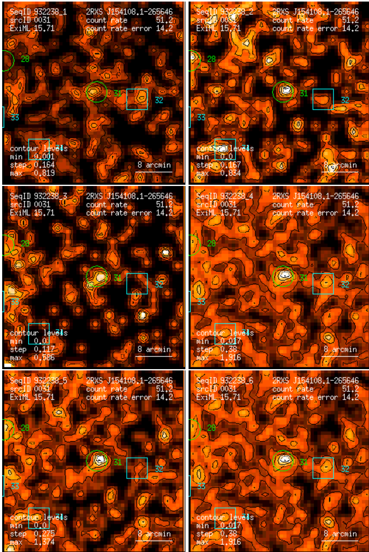
Figure 31: RASS 932238: detection 0031: band rate images, Gaussian filter: (1) PSPC channels 11 – 41, (2) 52 – 90, (3) 91 – 201, (4) 11 – 235, (5) 52 – 201, (6) 11 – 201. Broad band rates in counts/ks. Band rate contour levels in counts/ks/arcmin 2 .
