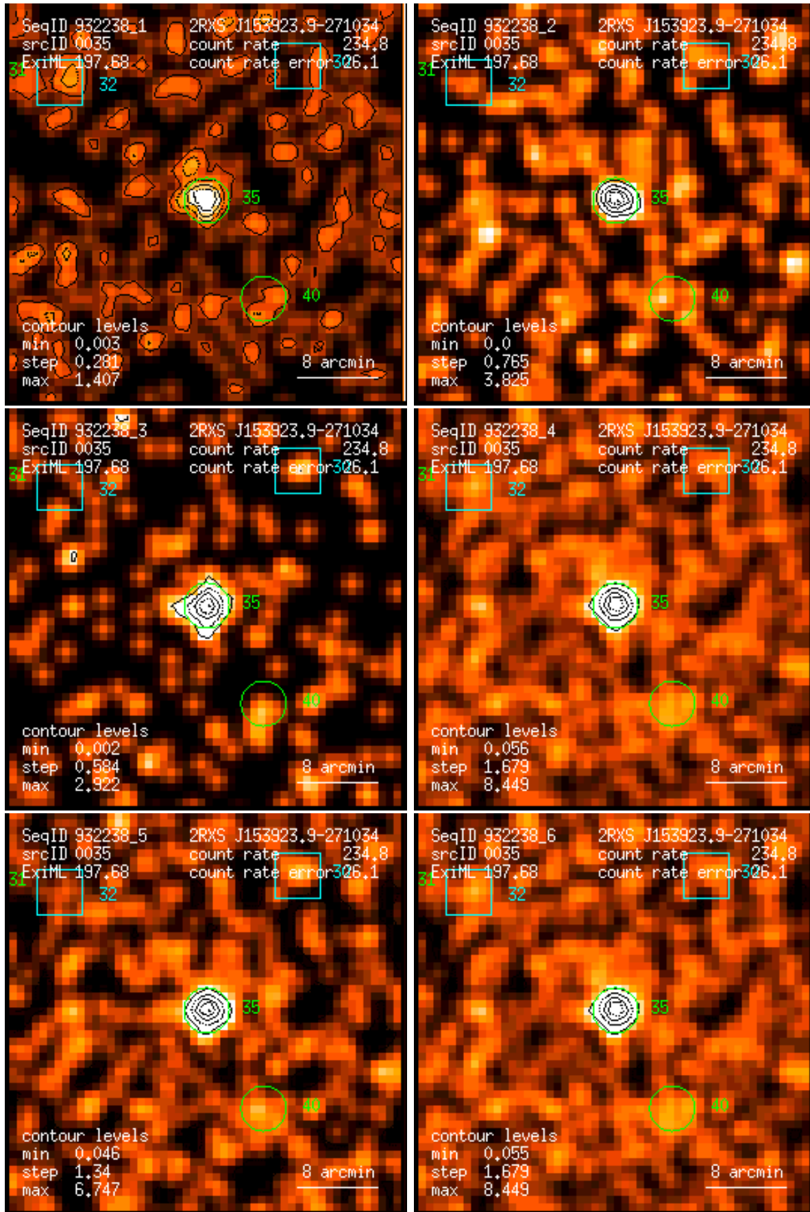
Figure 35: RASS 932238: detection 0035: band rate images, Gaussian filter: (1) PSPC channels 11 – 41, (2) 52 – 90, (3) 91 – 201, (4) 11 – 235, (5) 52 – 201, (6) 11 – 201. Broad band rates in counts/ks. Band rate contour levels in counts/ks/arcmin 2 .
